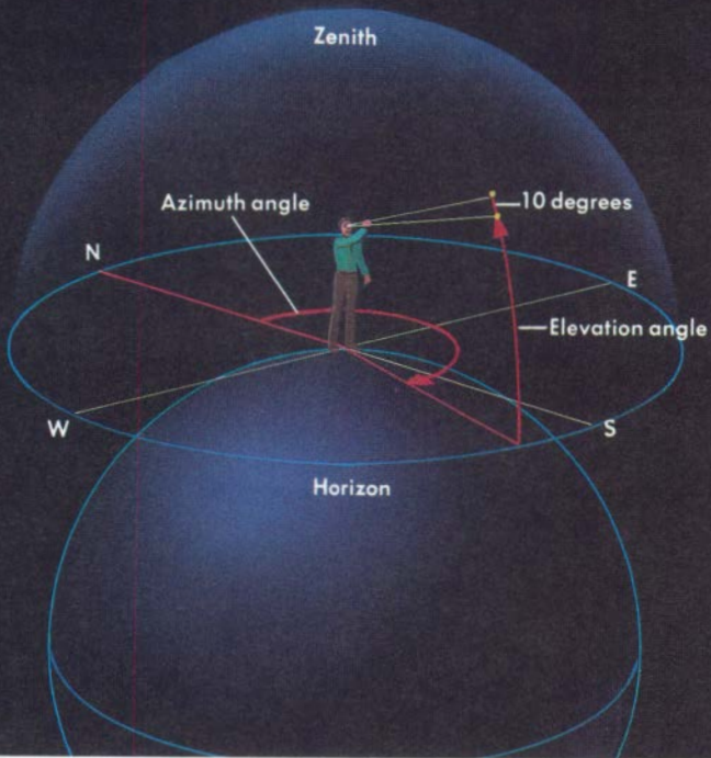
An observer and the horizon
