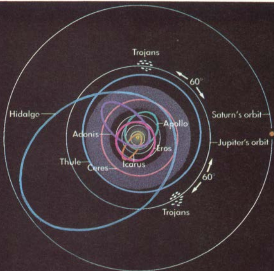
Asteroid orbits
