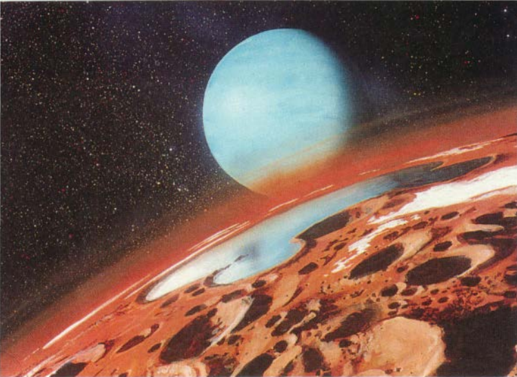
Neptune as seen from the surface of Triton
