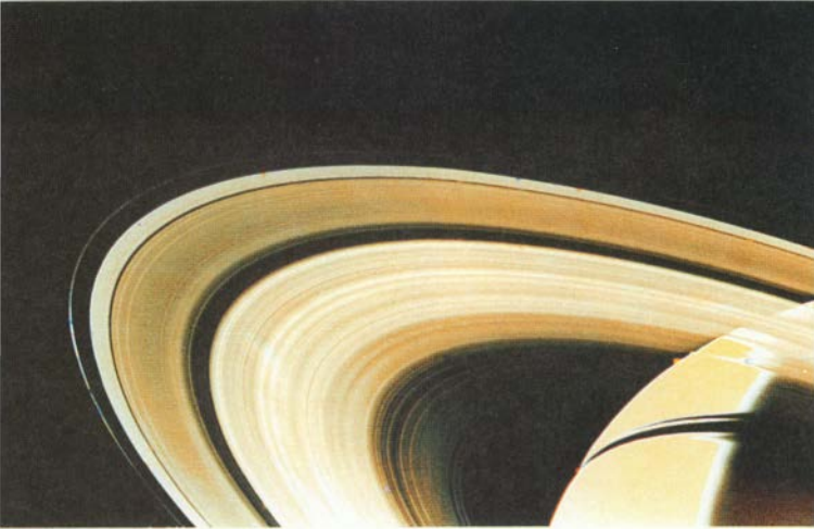
Rings showing "spokes" NASA
