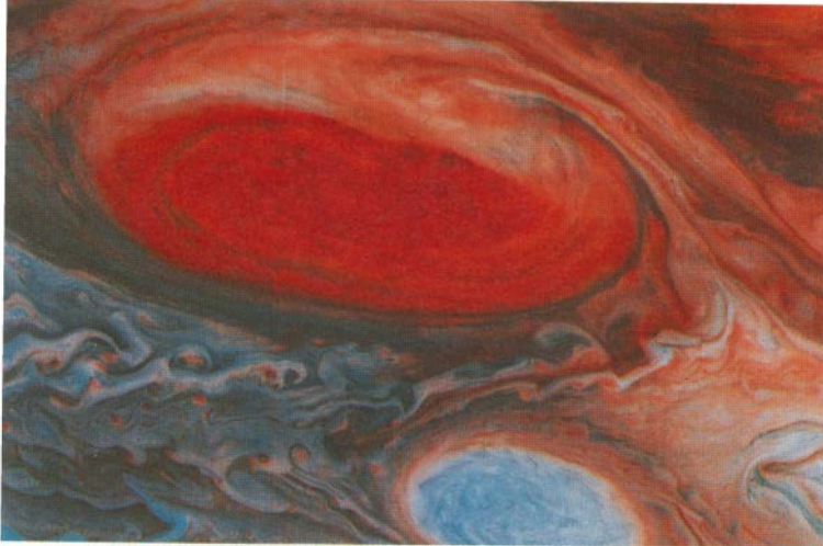
The Great Red Spot on Jupiter, as seen by Voyager 1 NASA
