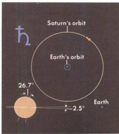
Saturn in orbit
