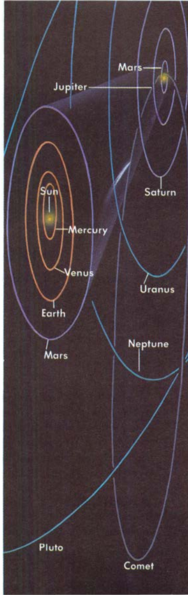
Planet orbits compared
