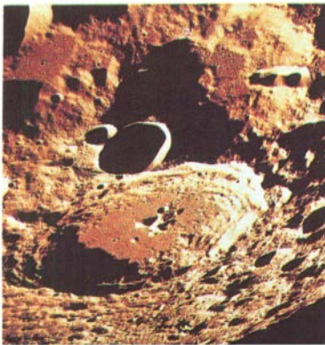
Lunar craters NASA
