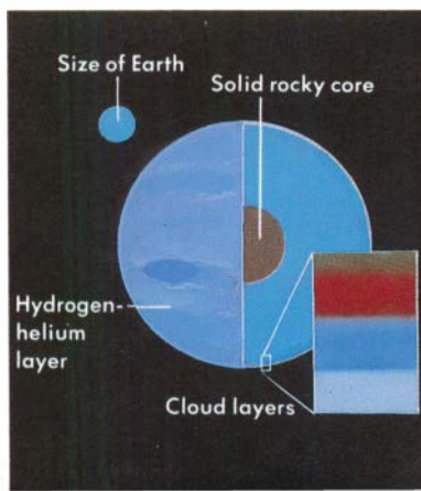
Neptune's structure
