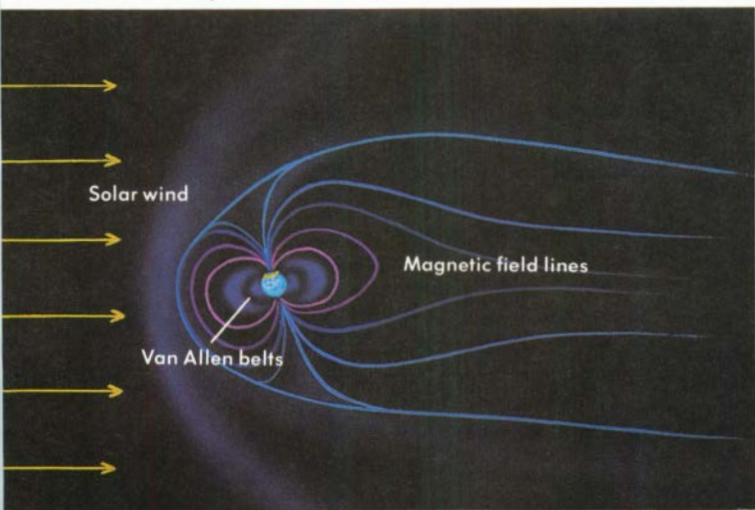
Earth and its magnetic field
