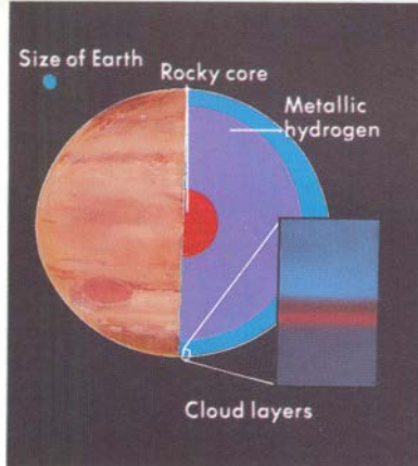
Structure of Jupiter
