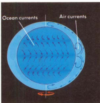
Atmospheric circulation patterns
