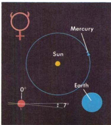
Mercury in orbit
