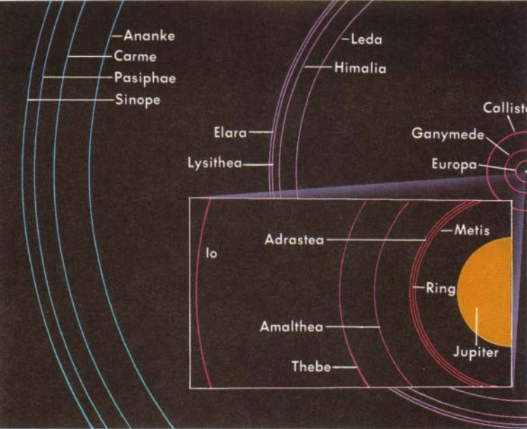
Orbits of Jupiter's satellites
