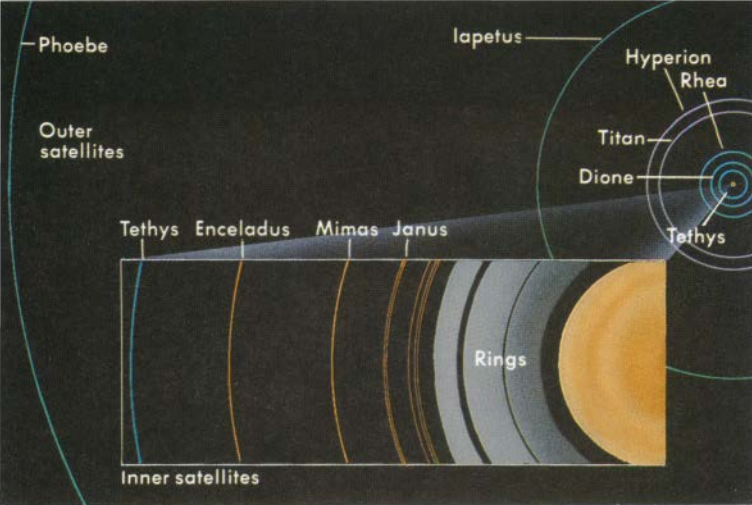
Orbits of Saturn's satellites
