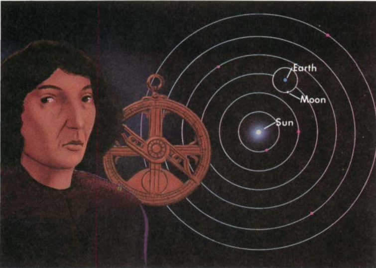
Copernicus' Sun-centered system
