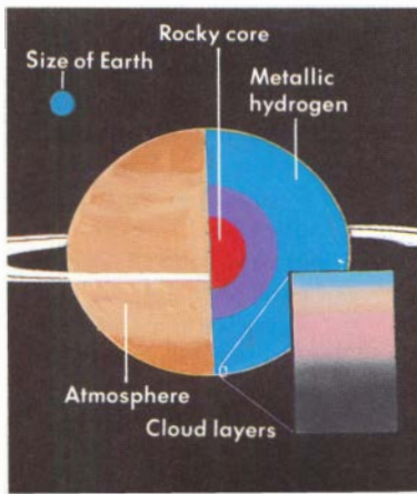
Internal structure of Saturn
