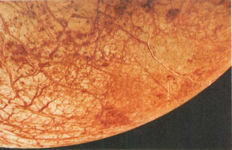
Close-up of Europa's surface NASA
