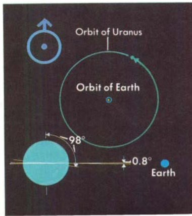
Uranus in orbit
