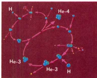
Nuclear fusion reaction
