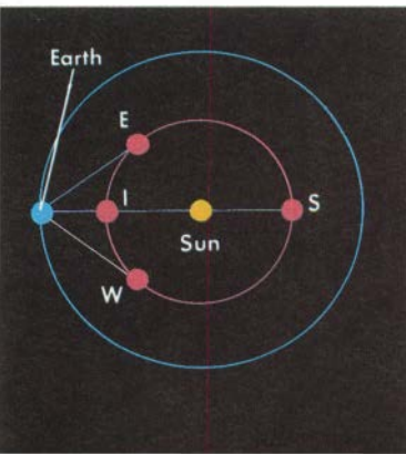
Inferior planet phenomena
