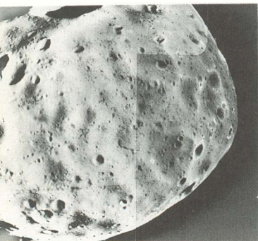
Phobos NASA
