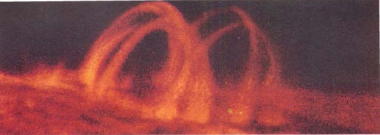
Prominences seen in X-ray light NASA
