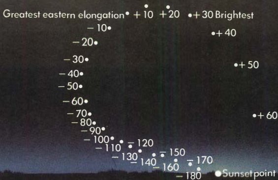
Finding chart for Venus in the evening sky 7/23/1992 to 3/30/1993
