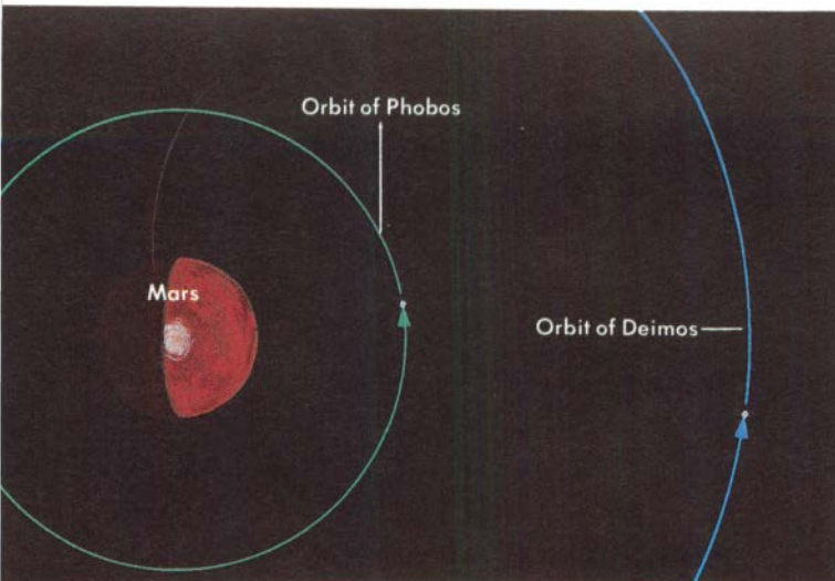
Orbits of Mars' satellites
