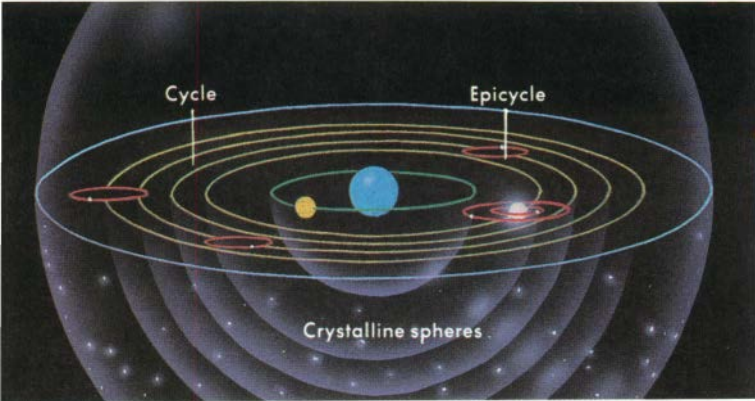
The Ptolemaic system
