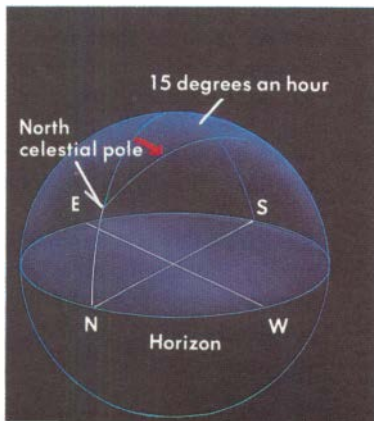
Sky motion around Earth
