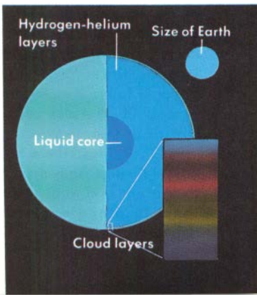
Structure of Uranus
