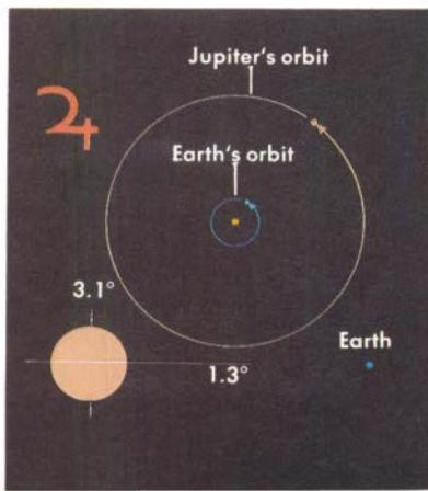
Jupiter in orbit
