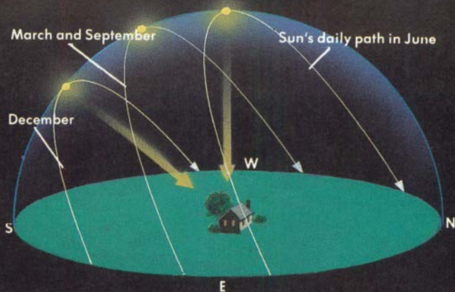
Sun's motion across the sky
