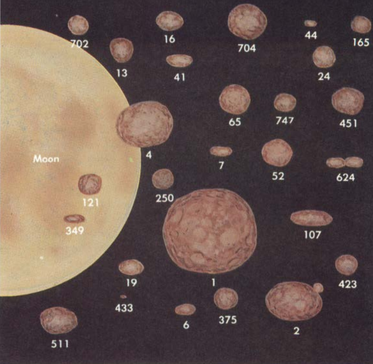
Some of the minor planets
