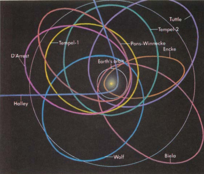
Some periodic comet orbits
