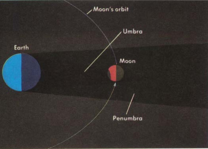
Geometry of a lunar eclipse
