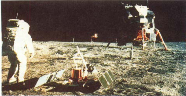
Apollo 11 astronauts on the Moon (1969) NASA
