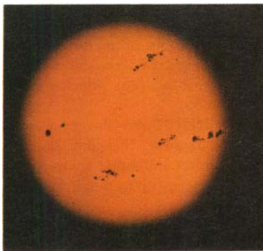
The Sun in red light NASA
