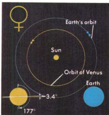
Venus in orbit
