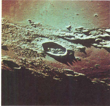
Lunar mountains NASA
