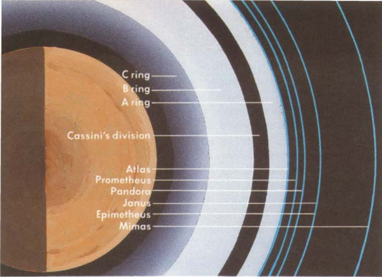
Saturn's rings
