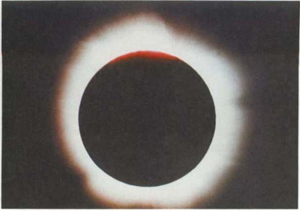
Total eclipse of the Sun NASA
