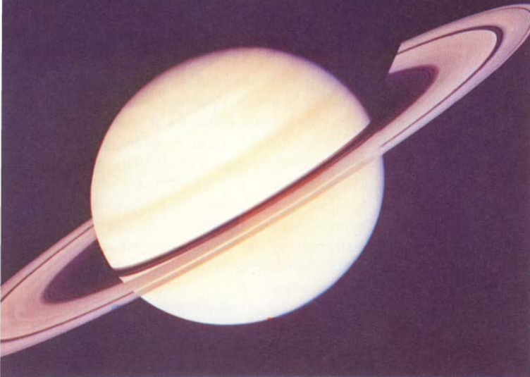
Saturn and its rings NASA
