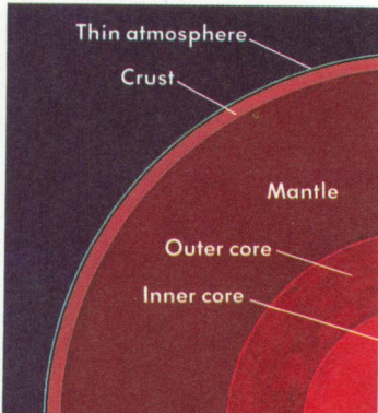
Terrestrial planet cross section
