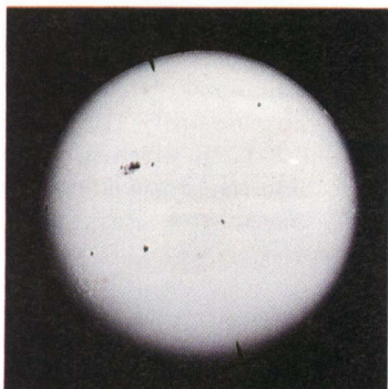
White-light image of the Sun NASA
