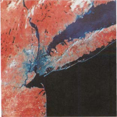
Landsat 4 photograph of Earth (1982) NASA
