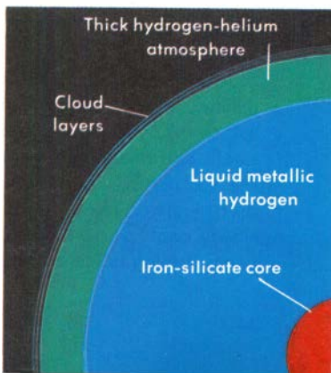
Jovian planet cross section
