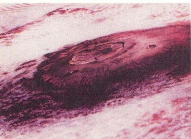
Olympus Mons NASA
