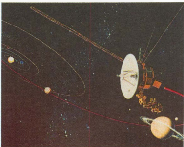
Voyager passing Saturn (1977) NASA
