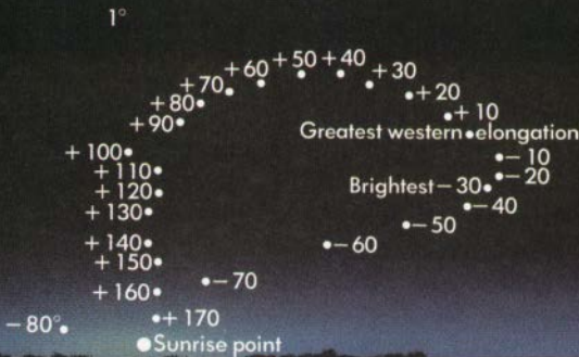
Finding chart for Venus in the morning sky 4/1 to 12/7, 1993
