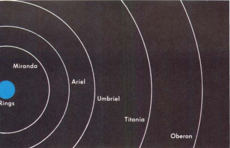
Orbits of Uranus' satellites
