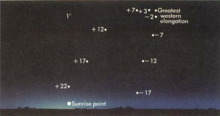
Finding chart for Mercury in the morning sky (above) and in the evening sky (opposite page)
