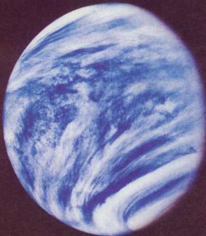
Venus seen by spacecraft in ultraviolet light NASA
