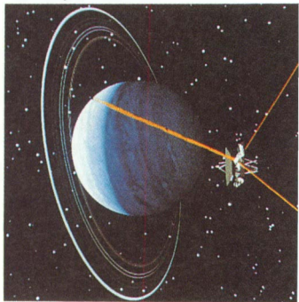
The rings of Uranus NASA
