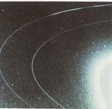
Neptune's rings NASA
