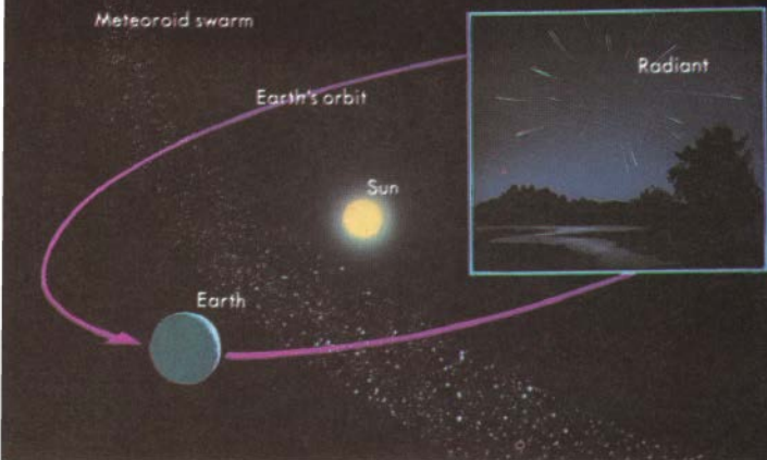
Meteoroid swarm crossing Earth's orbit
