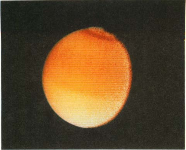
Titan NASA
