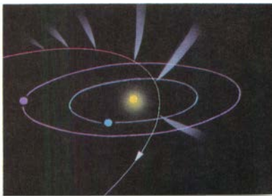
Comet tails point away from the Sun
