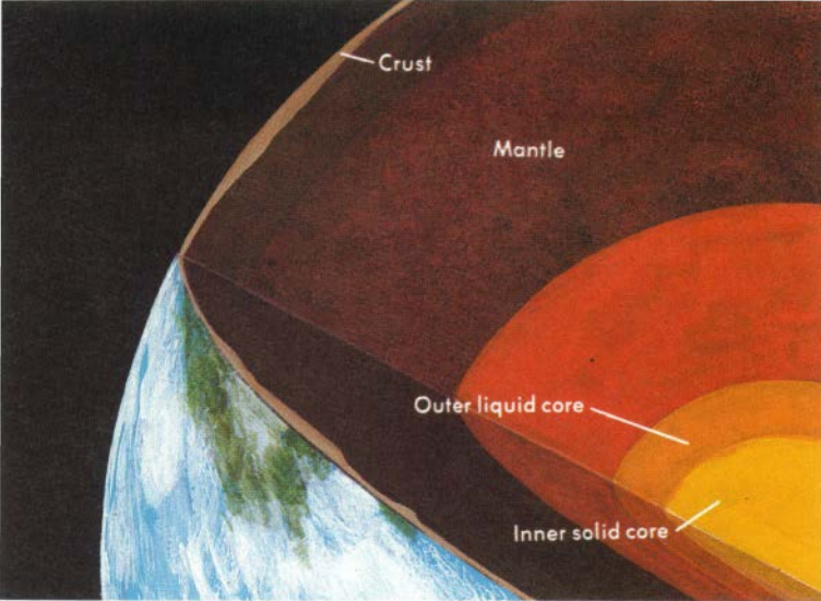
Earth's internal structure
