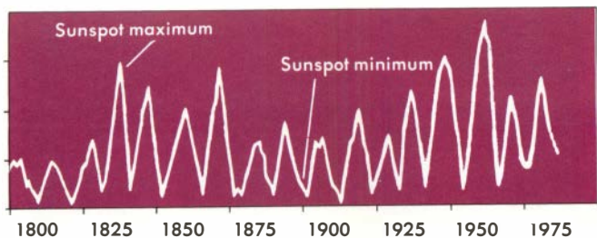
The sunspot cycle
