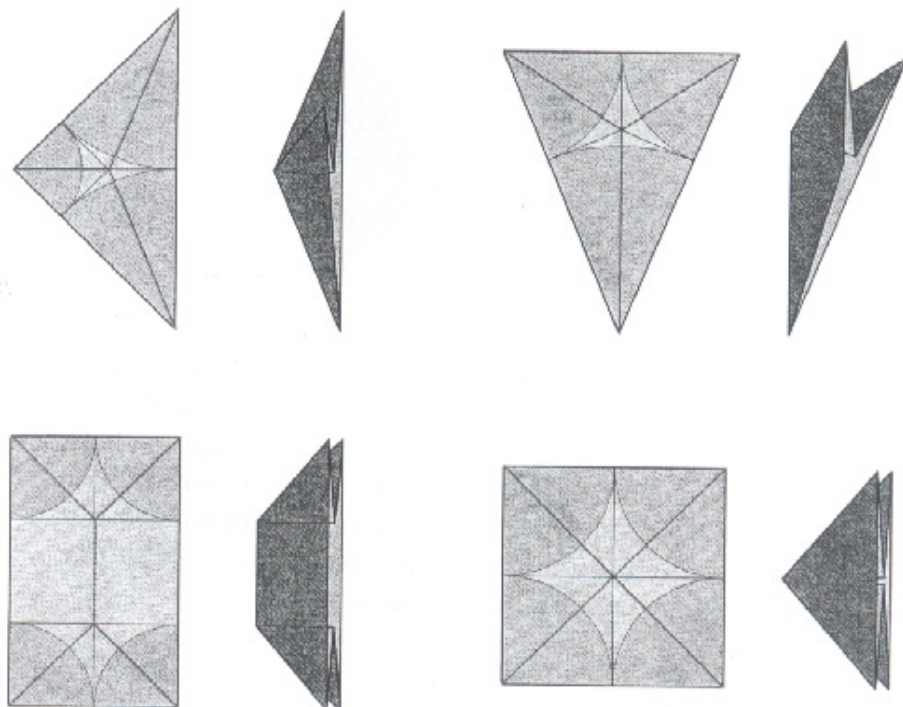
Figure 8.15. Four tiles decorated with circular arcs and their folded forms.
