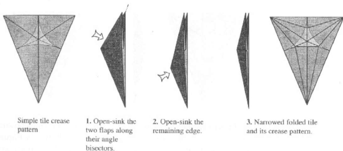
Figure 8.32. Procedure to narrow a tile using angled sink folds.
