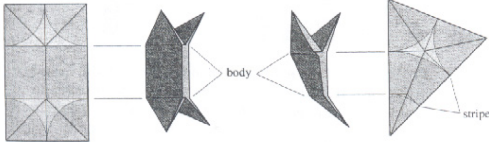
Figure 8.22. A body can be inserted into a triangular tile by representing it as a partial annulus.
