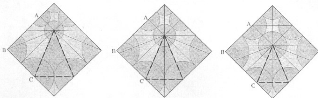
Figure 13.12. Three different ratio embeddings of the grafted Kite Base.
