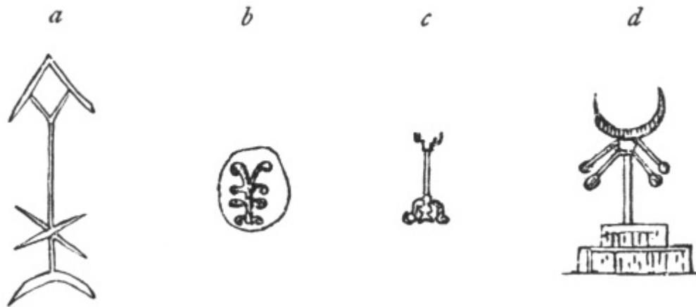
FIG. 61. RUDIMENTARY FORMS OF THE SACRED TREE [*1]
