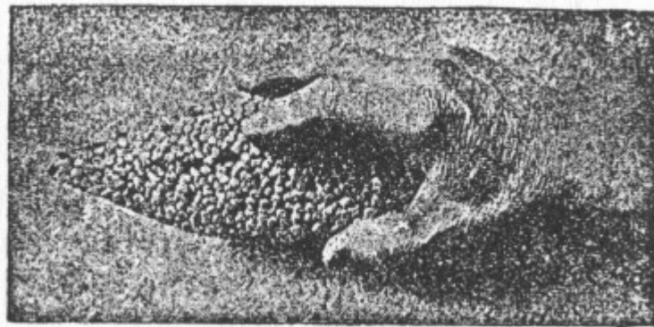
FIG. 80. INFLORESCENCE OF THE MALE DATE-PALM.
