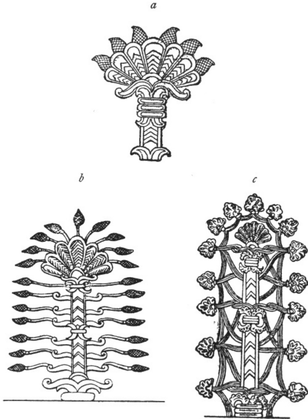
FIG. 63. CONVENTIONAL TREES OF ASSYRIAN BAS-RELIEFS.
