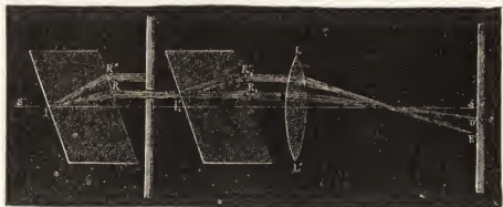
Fig. 179. The Polarizer and Analyzer.
