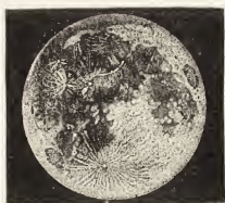
Fig 158. The Full moon.
