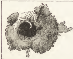
Fig. 183. A Solar Cyclone. May 5, 1857 (Secchi).
