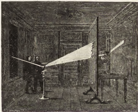
Fig. 129. Decomposition of Light by the Prism.
