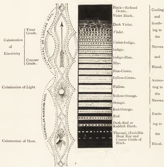
Fig. 131. The Solar Spectrum Analyzed and Systematized.
