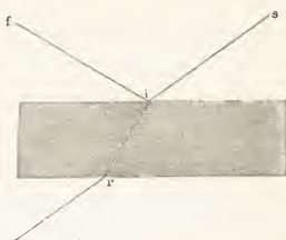
Fig. 172. Refraction and Reflection.
