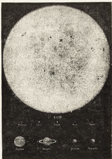
Fig. 157. Comparative sizes of the Sun and Planets after Guillemin, with a view of some of the spots and mottled appearance of sun.
