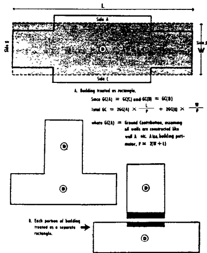
FIGURE 12.—Perimeter effects.
