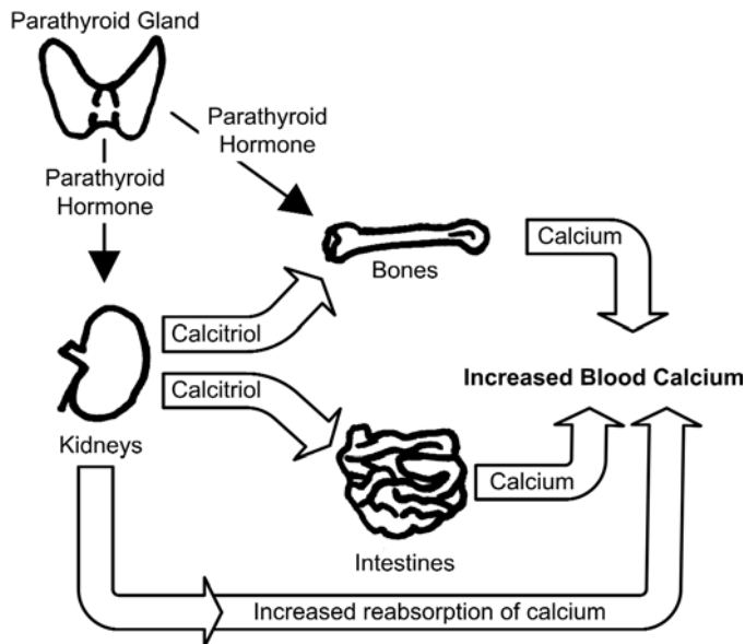
Figure 9-3 Calcium regulation.
