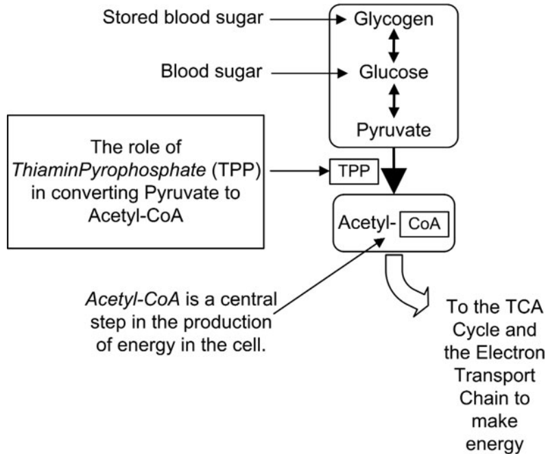
Figure 1-3 The role of thiamin in energy production.
