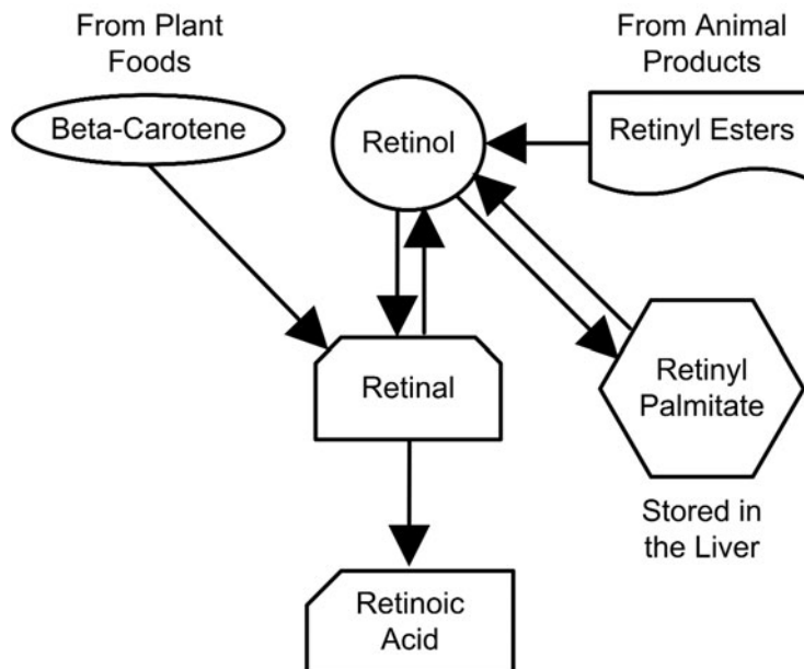
Figure 3-1 The forms of vitamin A.
