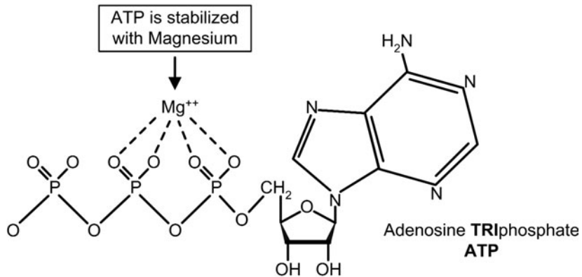
Figure 10-6 ATP is stabilized with magnesium.
