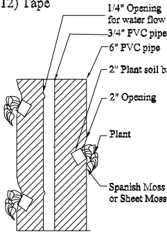
Cross Section of Assembly
