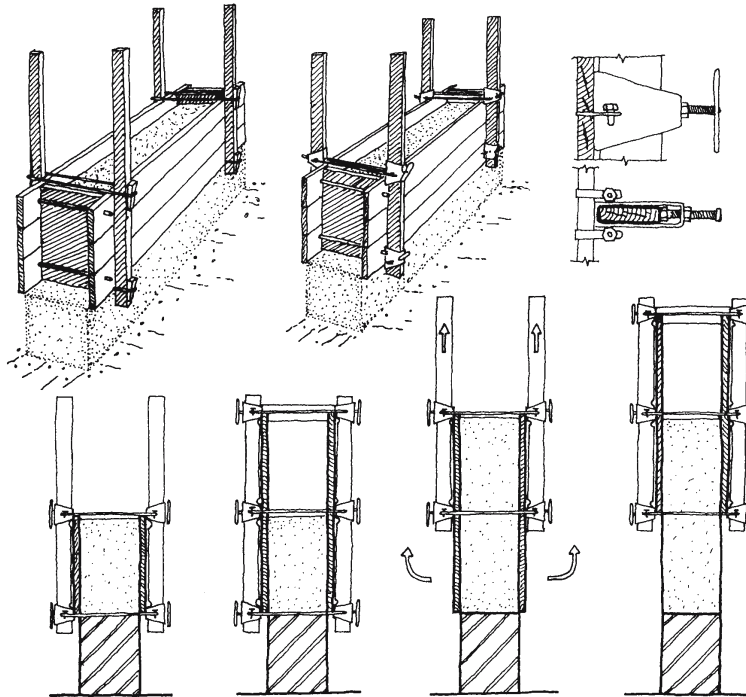
5.3 Formwork without intermediary spacers
