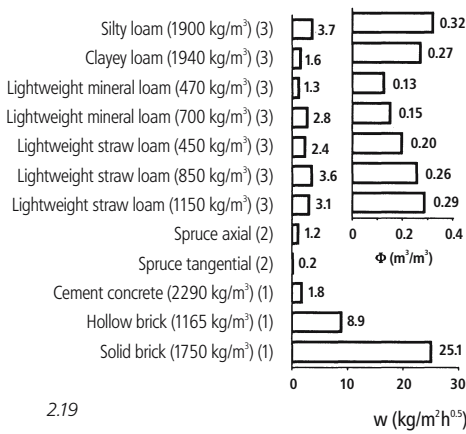
2.19 Water absorption coefficient 'w' of loams in comparison with common building materials 2.20 Water absorption curves of loams
