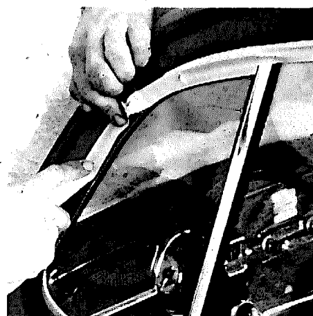
A taped-paper dispenser will make the masking job faster and easier.
