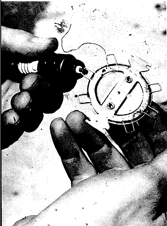
Sparkplugs should be gapped to specifications with a special wire gauge.
