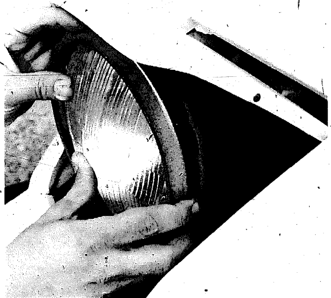
Having removed three screws, you can now remove the headlight retaining ring.
