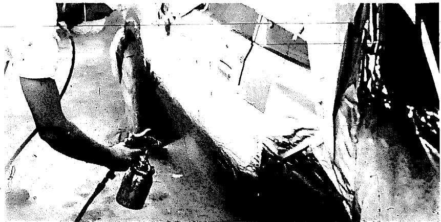
If you aren't going to paint the wheels, make up a cloth or plastic wheel cover and move it from wheel to wheel.
