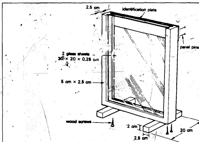
Diagram #1 Wormery (Rothemann pattern) Final of study 6.2
