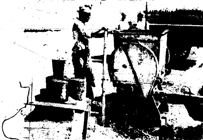
A DOUGH-MIXER used for adobe brick making. The interior blades are rotated by means of a gasoline engine.
