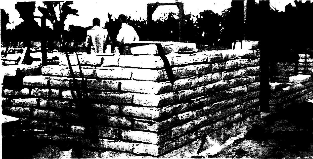
ADOBE-HOUSE CONSTRUCTION, showing brick arrangement, vertical reinforcing steel, and door frames in place.
