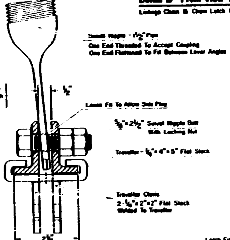
Detail C - Traveler and Swivel Side View Scale: Full Size
