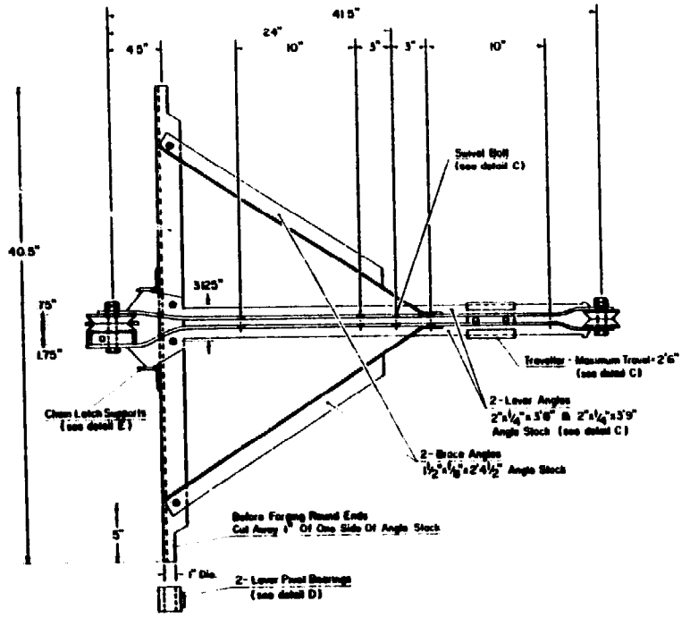
Top View - Assembly Linkage Chain & Chain Latch Omitted Scale: 3/8" = 1 foot
