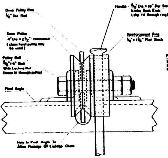
Detail B - From View 'A' - Drive Pulley Linkage Chain & Chain Latch Omitted Scale: Full Size
