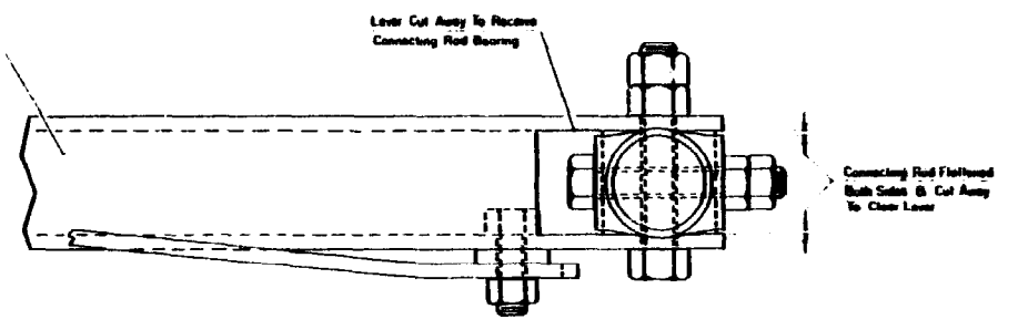
Top View - Lever End Pivot
