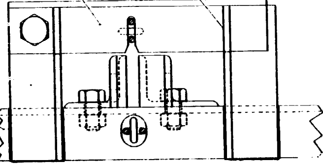
Detail E - From View 'A' - Linkage Chain Latch Drive Pulley Omitted
