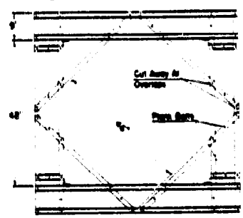
Section View A-A Platform Constructed Of 1\frac{1}{2} " x 1\frac{1}{2} " Angle Steel And \frac{1}{2} " Bars With 2-66" & 2-48" Wood Planks
