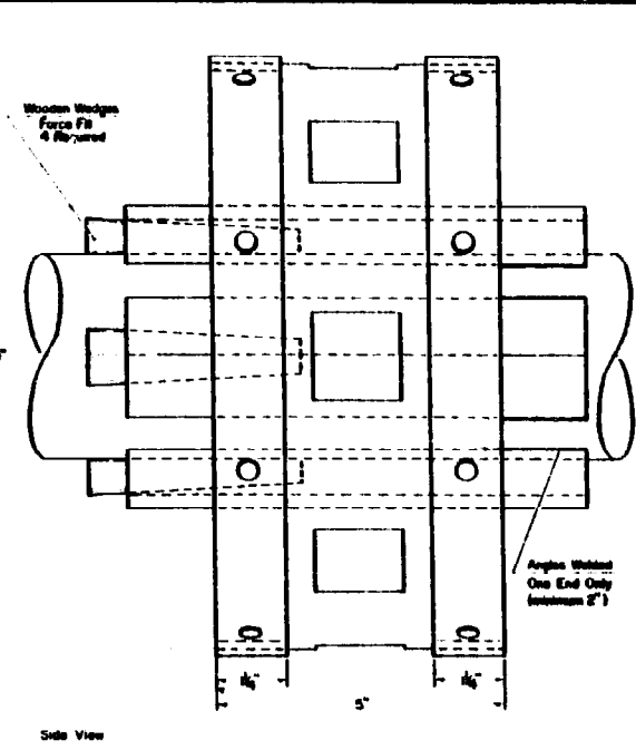
Hub Assembly Scale Full Size
