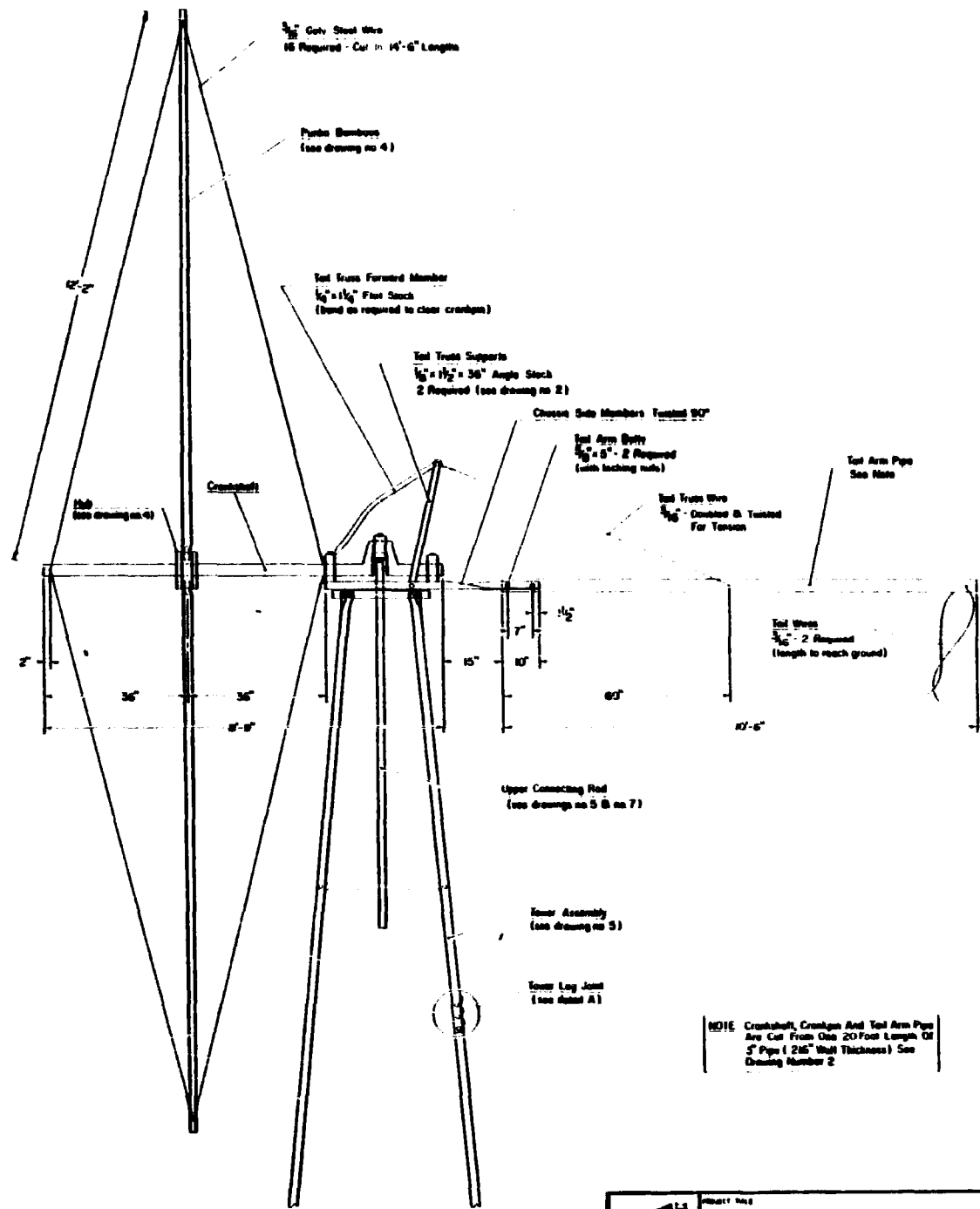
Side View - Pusher and Tail Arm Assembly
