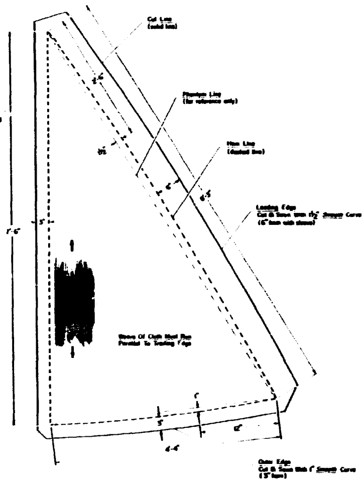
Soil Cutting Pattern 8 Required Scale Inches = 1 foot
