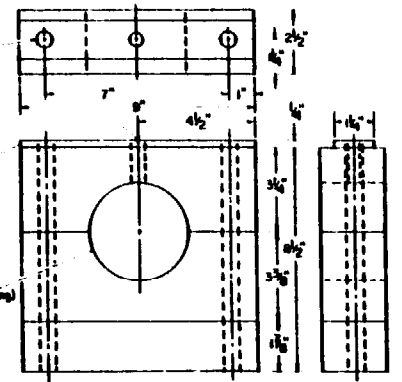
Detail A - Main Bearing 2 - Required Hardwood Scale: Half Size
