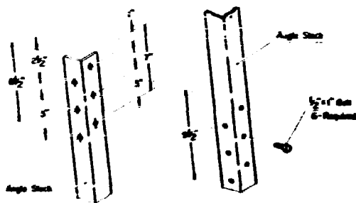
Detail A - Tower Leg Joint As Required
