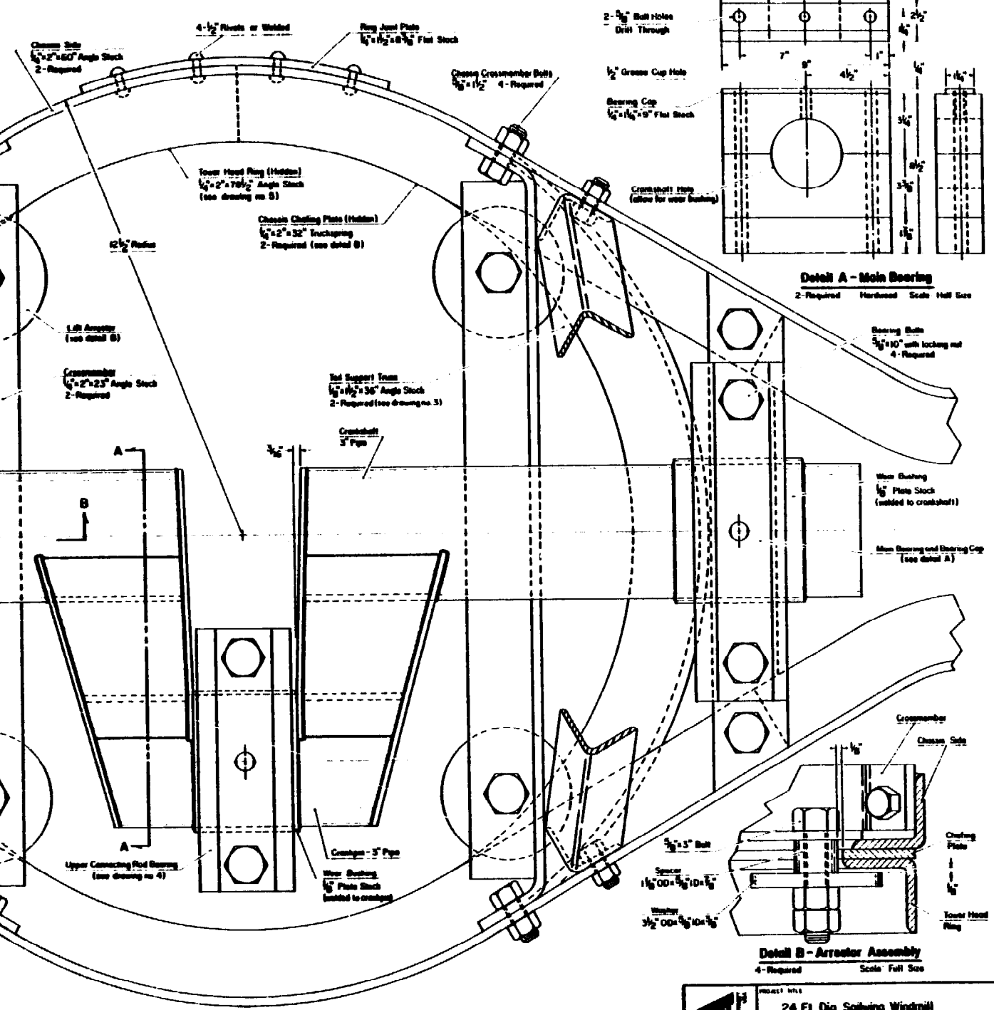
Top View - Reciprocating Chassis Assembly
