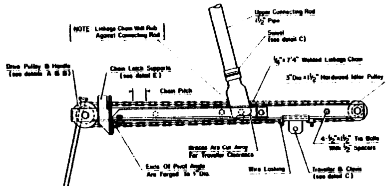
Side View - Assembly Chain Latch Omitted Scale: 3/8" = 1 foot
