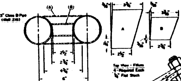
Section View A-A and Fillets Scale: Half Size
