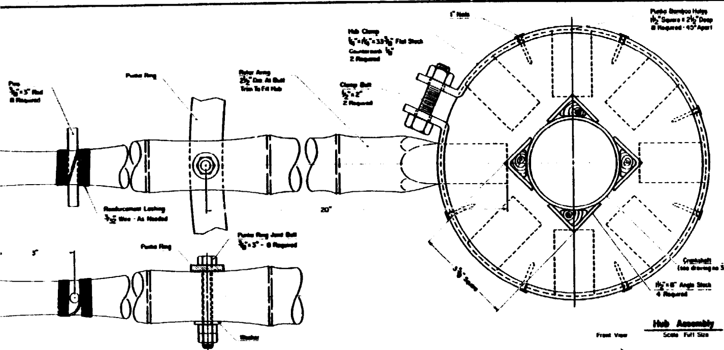
Top View - Bamboo Tip And Puntia Ring Joint Scale Full Size
