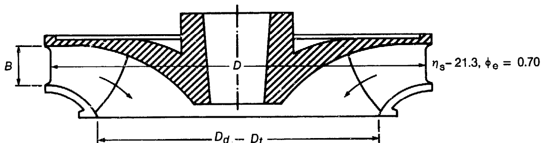
Figura 3 Rotor Típico de Turbina Figure 3 Typical Turbine Runner
