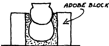
CROSS-SECTION, FIREBOX
