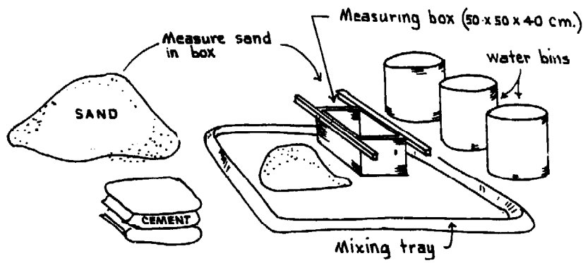
Fig. 15 Mixing the Concrete by Hand
