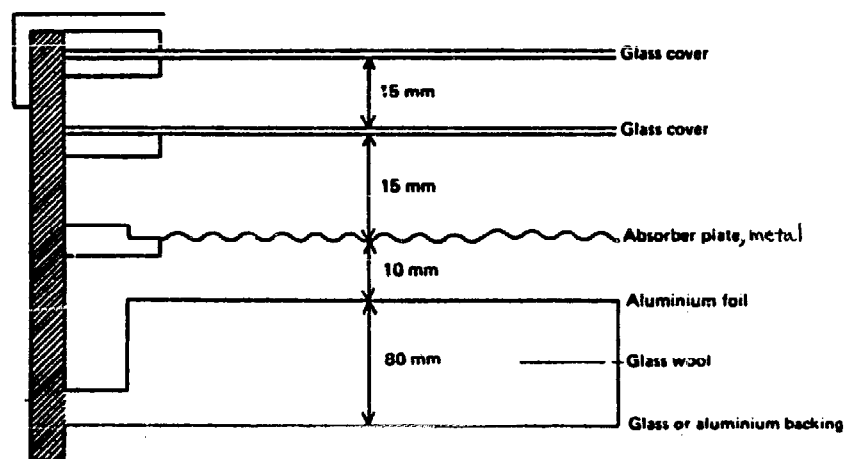
cross section
