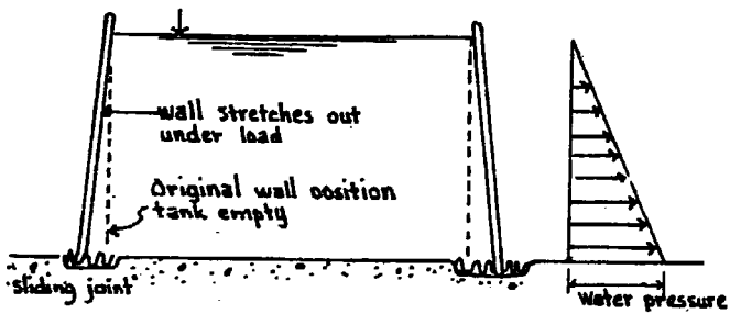
Fig. 7 WALLS FREE TO MOVE
