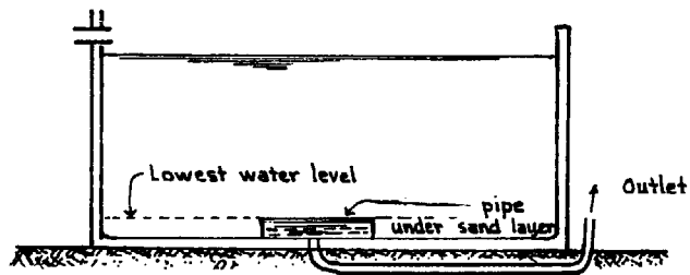
Fig. 14 - SLOW SAND FILTER IN TANK OVER OUTLET
