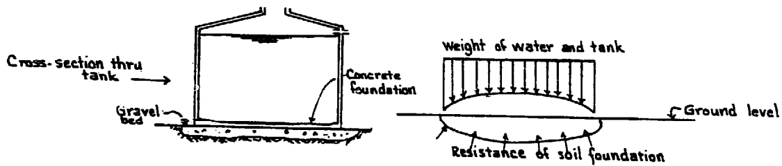
Fig. 5 FOUNDATION OF SMALL TANK - WALLS AND BASE JOINED
