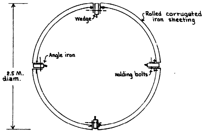
top view of formwork
