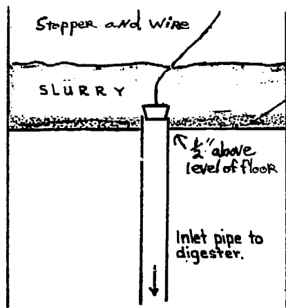
SINK TRAP
