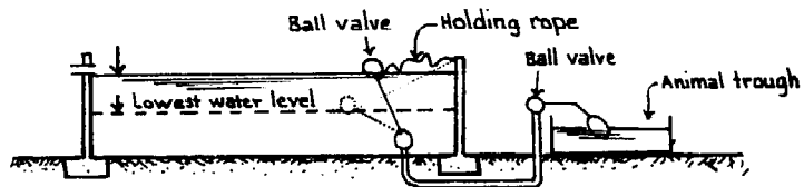
Fig. 13 - Ball valves for cattle watering
