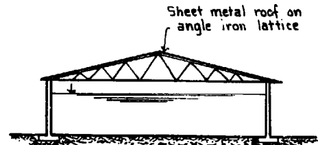
Fig. 12 - ROOF FOR LARGER TANK
