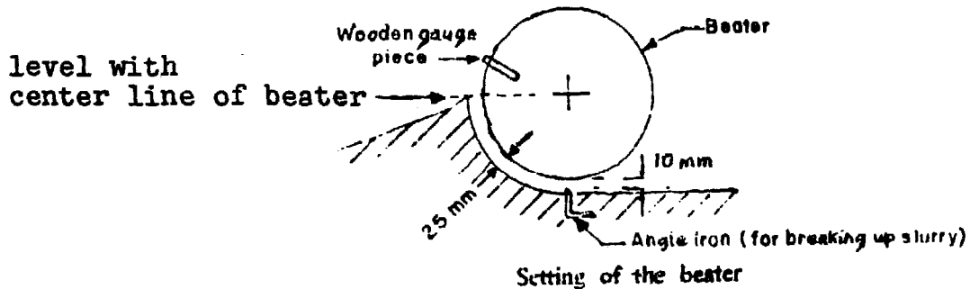
Slurry-mixing machine
