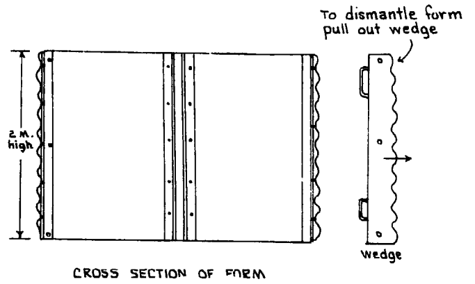
CROSS SECTION OF FORM
