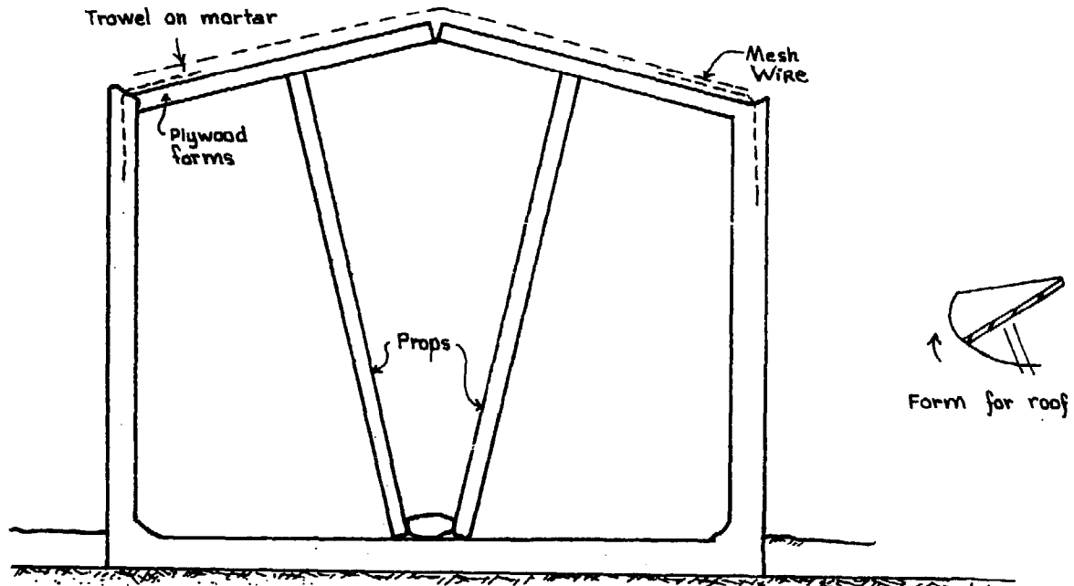
Figure 31. Constructing the Roof
