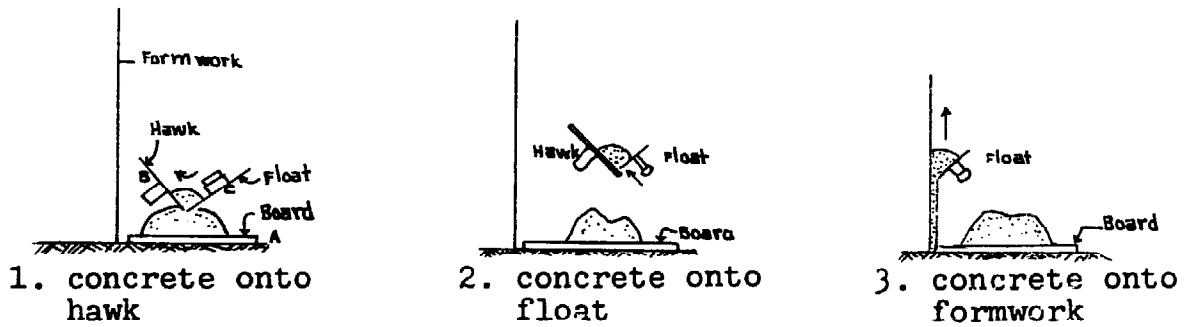
Fig. 17 Trowelling the Concrete onto the Formwork
