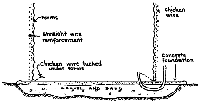
Fig. 21 Erecting Formwork and winding on reinforcing wire
