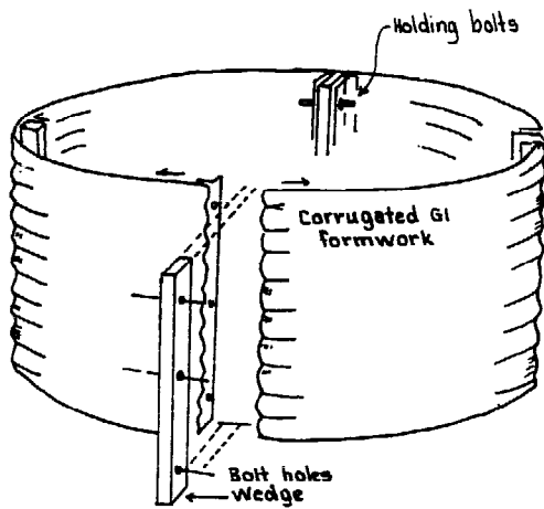
FIG. 19. ASSEMBLING THE FORMWORK
