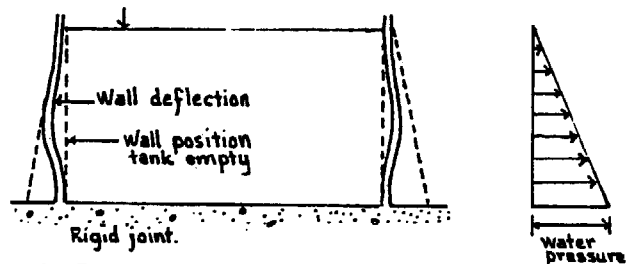
Fig. 8 WALLS JOINED WITH FLOOR
