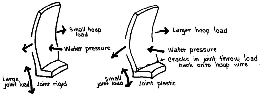
Fig. 9 - How the loads are taken
