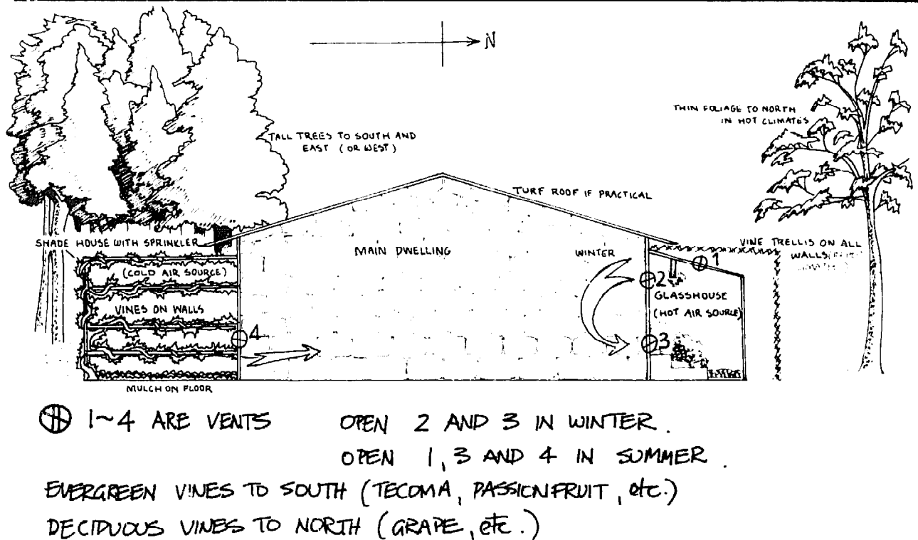
FIG. 6.2: HOUSE MODIFIED BY ATTACHED SHADE HOUSE AND GREENHOUSE, TRELLIS, VINES. SEE ALSO REFS. 8 AND 24.
