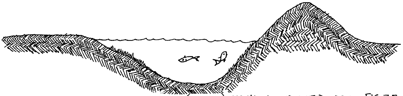
TYPICAL EARBANKS OF FLATLANDS (SECTION). USUALLY UNPLANTED, OPEN TO WIND AND EVAPORATION. OFTEN WASTE SUBSOIL IS HEAPED ON THE SUN SIDE AND STOCK CAN APPROACH FROM ANY QUARTER MUDDING WATER. FIG. 7.5
