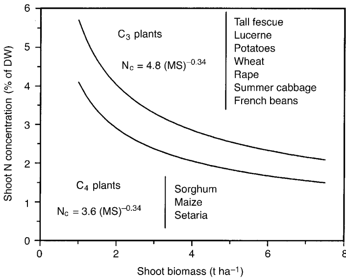
Fig. 2.3. Critical nitrogen concentration (N c ) for several C 3 and C 4 species. Each reference curve is fitted to an allometric relationship where MS stands for shoot biomass (t ha -1 ). DW, dry weight.
