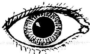
NORMAL EYE
