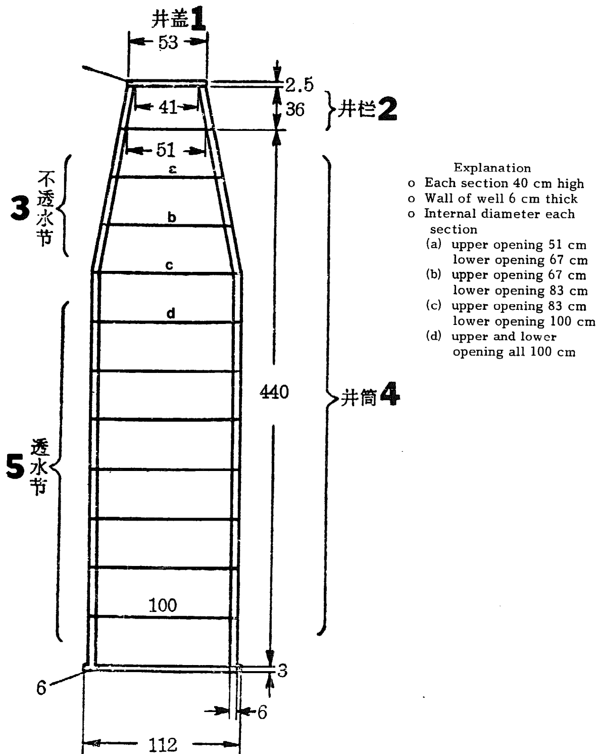
Figure 14. Simple drawing of cement tile barrel well.
