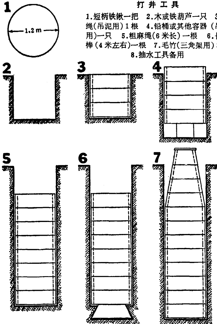
Figure 16. Diagram for procedure of digging cement tile barrel well.
