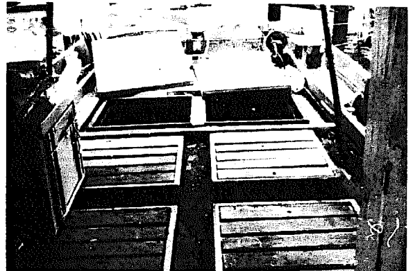
Fig. 5. View of Sandra Ann 's deck space looking aft from door of the house. The four live wells are shown in the foreground with the slatted covers in place. The main fish hold (hatch covers removed) is behind the live wells. Box with the stove is at left. Note the long unobstructed working space extending aft.
