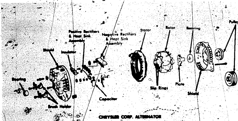
CHRYSLER CORP. ALTERNATOR
