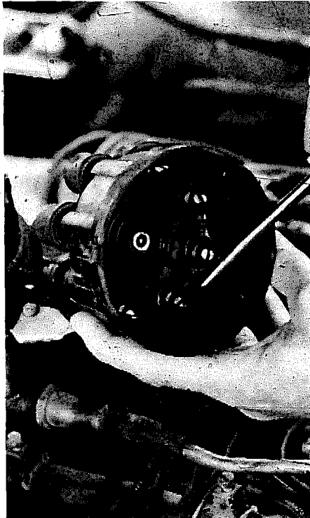
Light carbon deposits should be scraped off distributor cap contacts. If there is heavy carbon build-up or cracks in the cap, it should be replaced.
