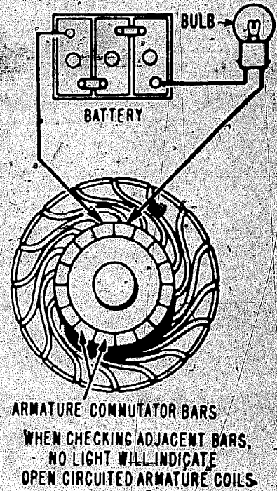
Generator armature test for open circuit. Same test can be used on starter armatures.
