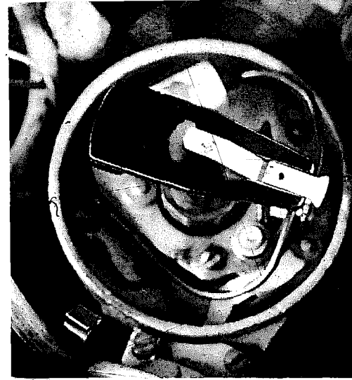
(left) GM-type rotor and distributor require slightly different service techniques than other distributors. (right) Non-GM distributor with rotor, points and condenser in place. Always note where the wires run from and connect to.
