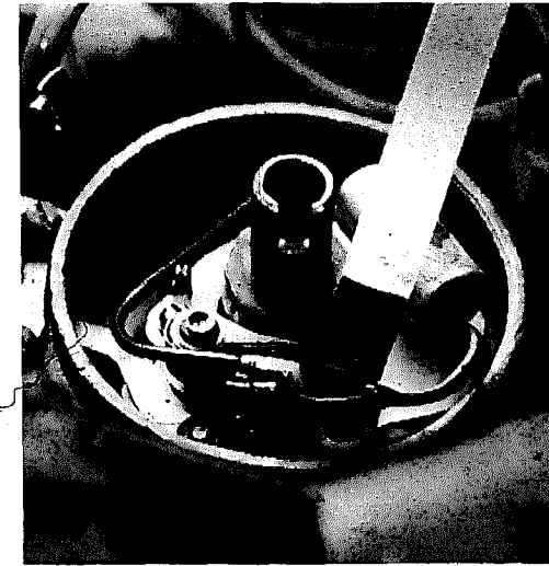
(left) To adjust the point gap, the rubbing block must be on a high lobe of the distributor cam. Some tuneup kits include a special ring that fits over the cam to hold the points open for gapping. (right) With the points held open by the cam, the gap can be adjusted to drag slightly on the specified feeler gauge. The adjustment slot is to the right of the feeler gauge and almost hidden by the wire from the condenser.
