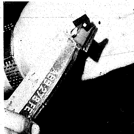
Newer disc pads come with this spring steel attachment that is supposed to rub against the rotor when the pad is worn down. The noise it produces will let you know you need brake work.
