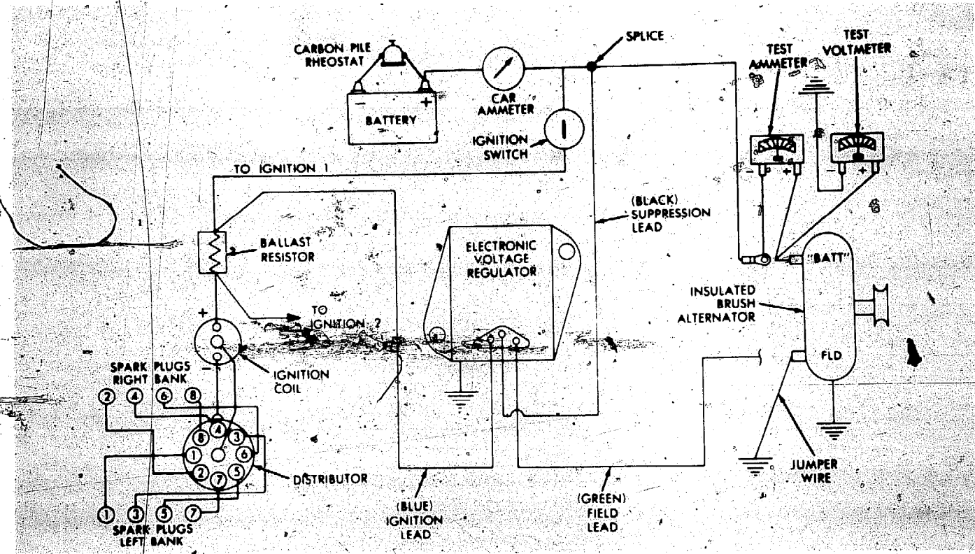
Schematic for current output test as mentioned in text.
