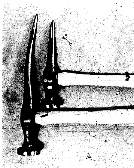
Dinging hammers come in different "reaches" or lengths so that if you have space limitations you can use the shorter, lighter one instead of fighting with the long one.
