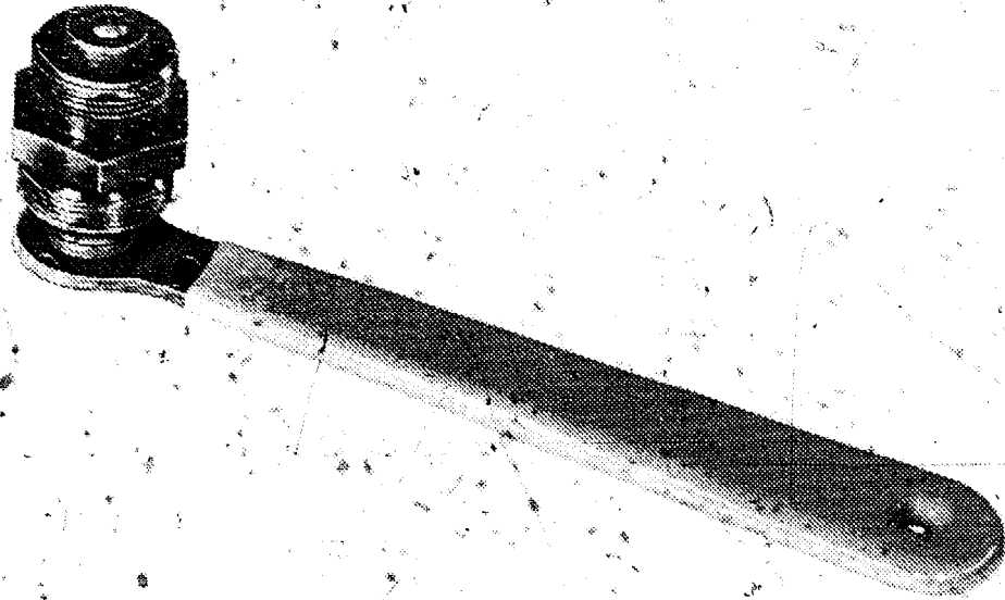
Fig. 5-47. A cotterless crank extractor tool.
