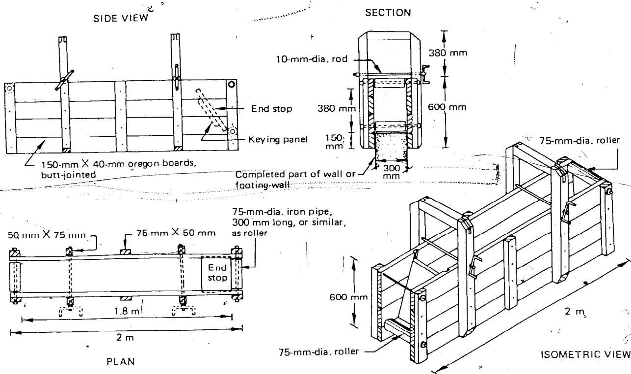
Details of crawler formwork
