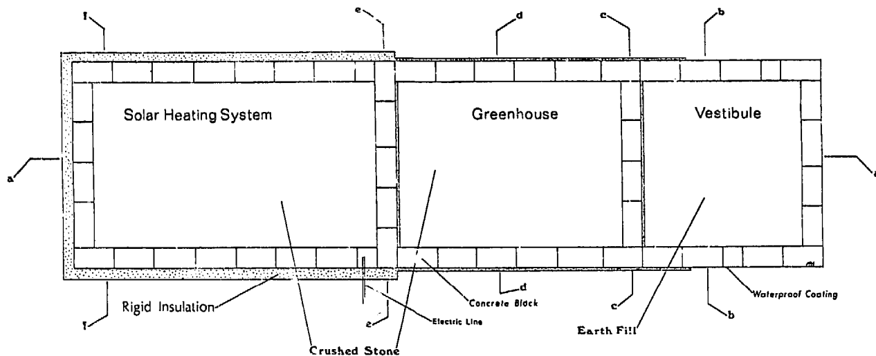
Scale 1:16 Cross Section at the Fourth Course
