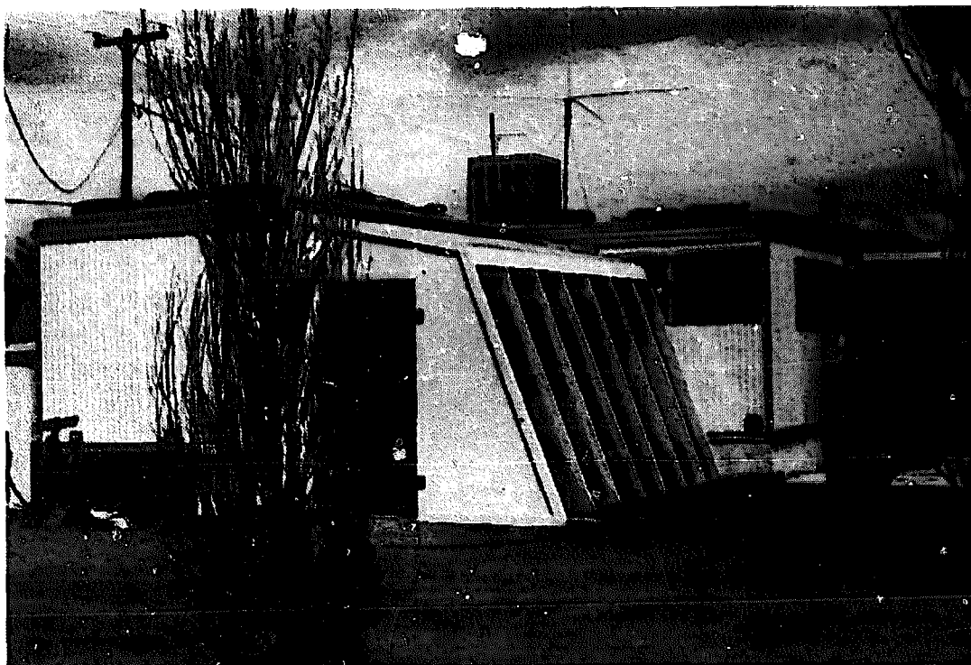
Greenhouse on Mobile Home. Built in Workshop by Mojave County Solar Energy Commission: Kingman, Arizona
