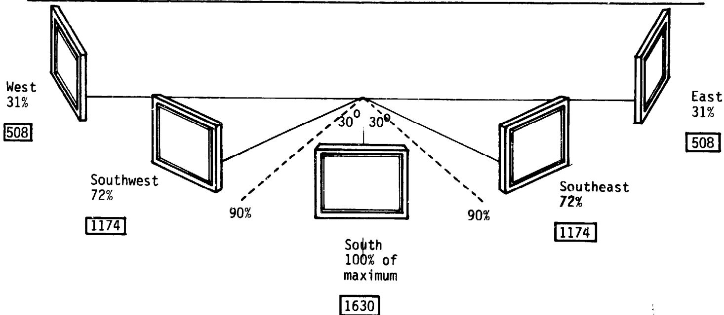
Figure 1. Solar radiation striking vertical wall relative to maximum southerly exposure (100 percent), winter condition, for the NORWESCAP latitude. Numbers in boxes represent average Btu per square foot per day solar energy striking the vertical wall in January.
