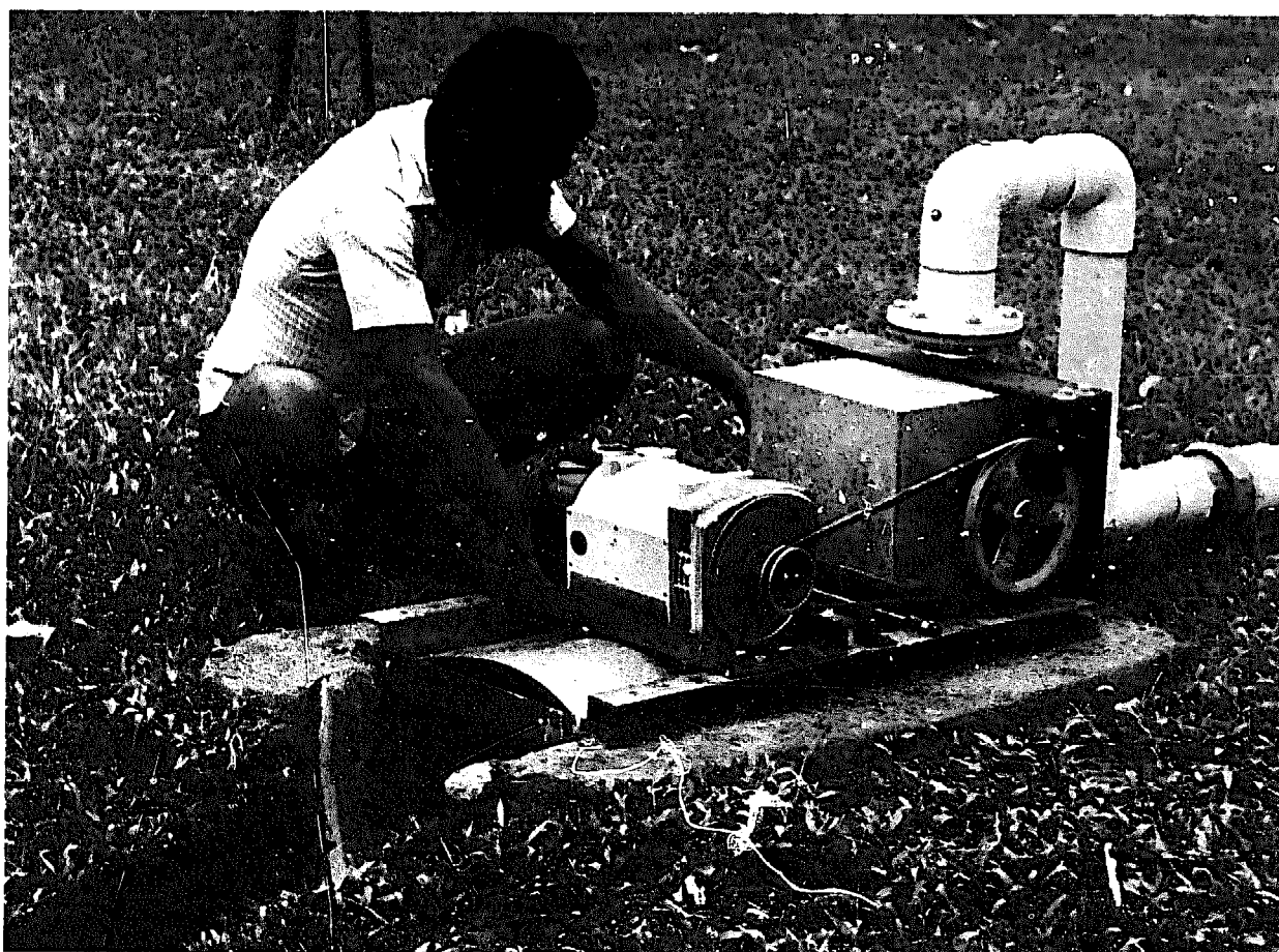
A 5 kW Pelton prototype designed at the Appropriate Technology Development Institute (Lae, PNG) for local fabrication and quick, trouble-free installation. A box can be used to protect the equipment from the elements.
