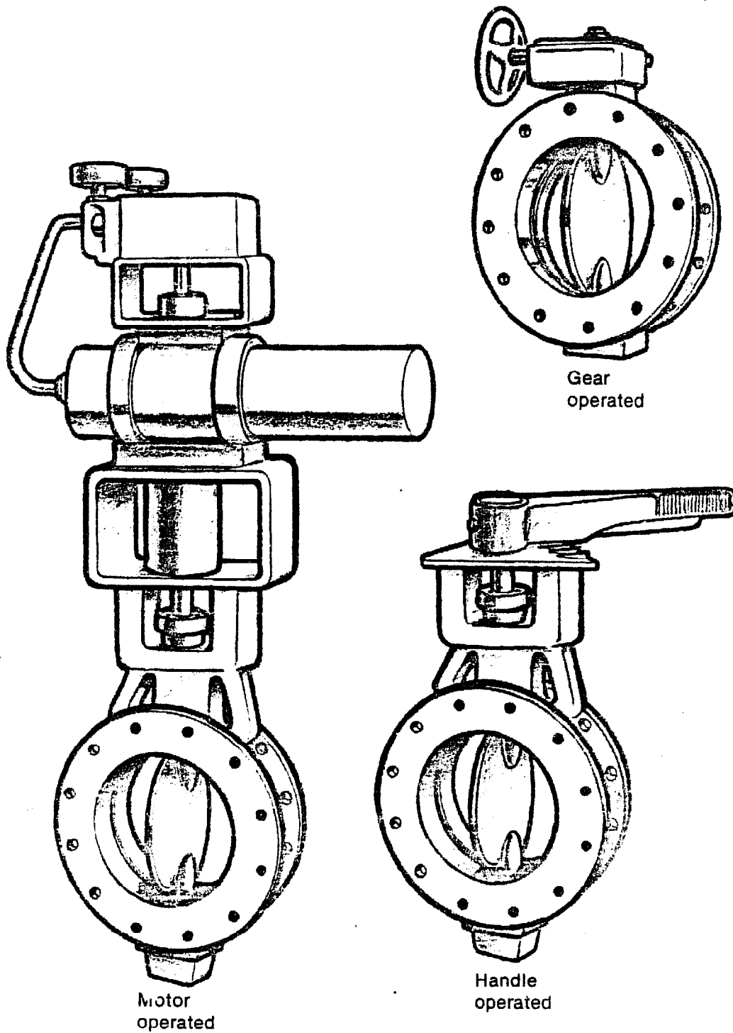
Figure 4.5-6. Butterfly valves.
