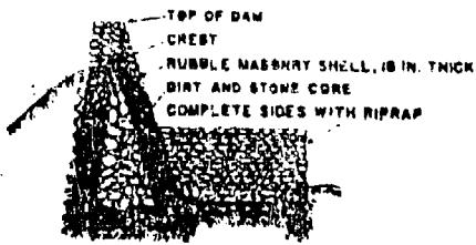
(C) RUBBLE MASONRY SPILLWAY
