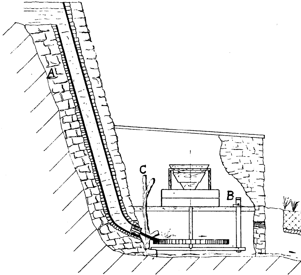
Fig. 1. Cretan water-mill.
