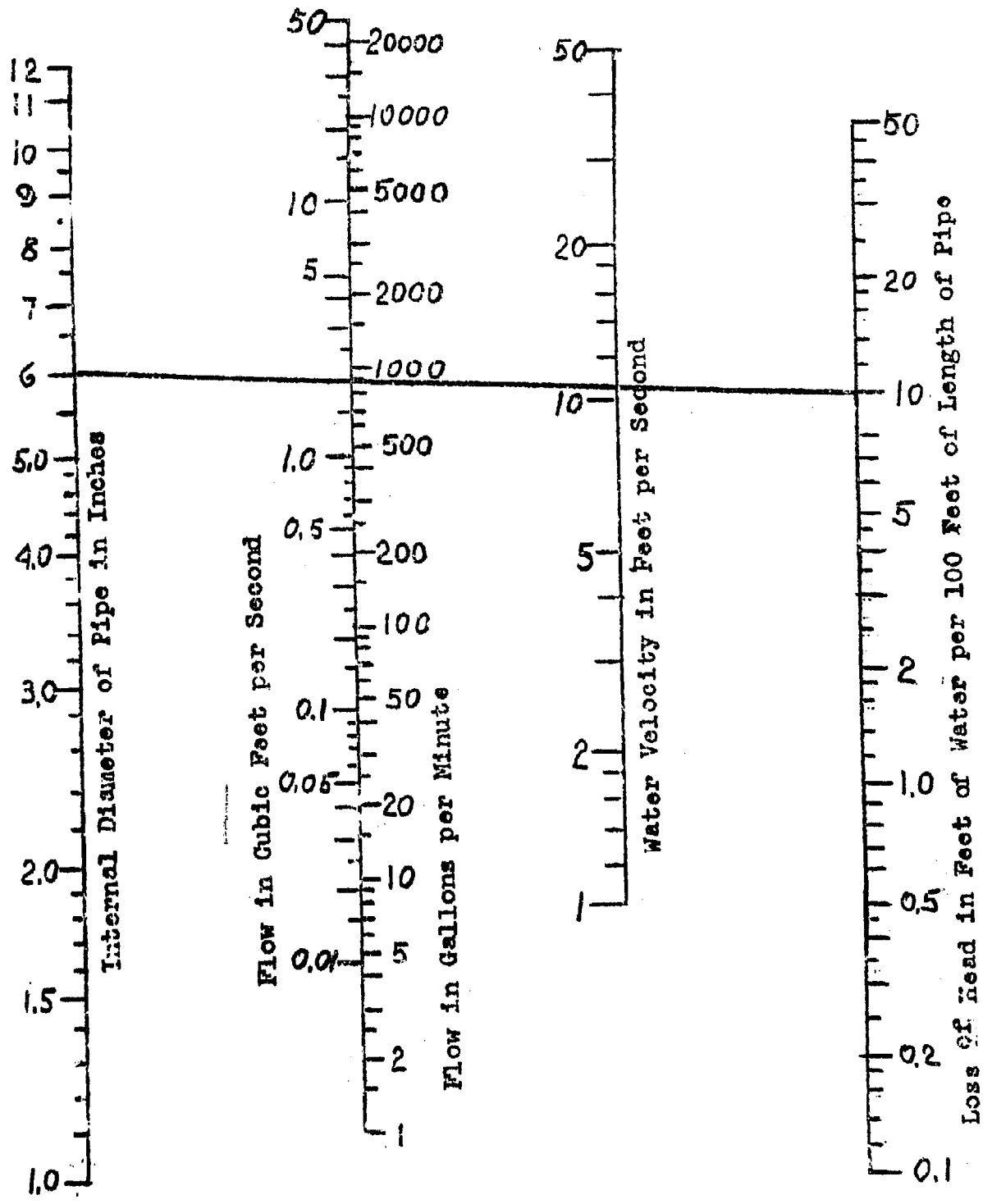
Figure 14. Nomograph for head loss in steel pipes
