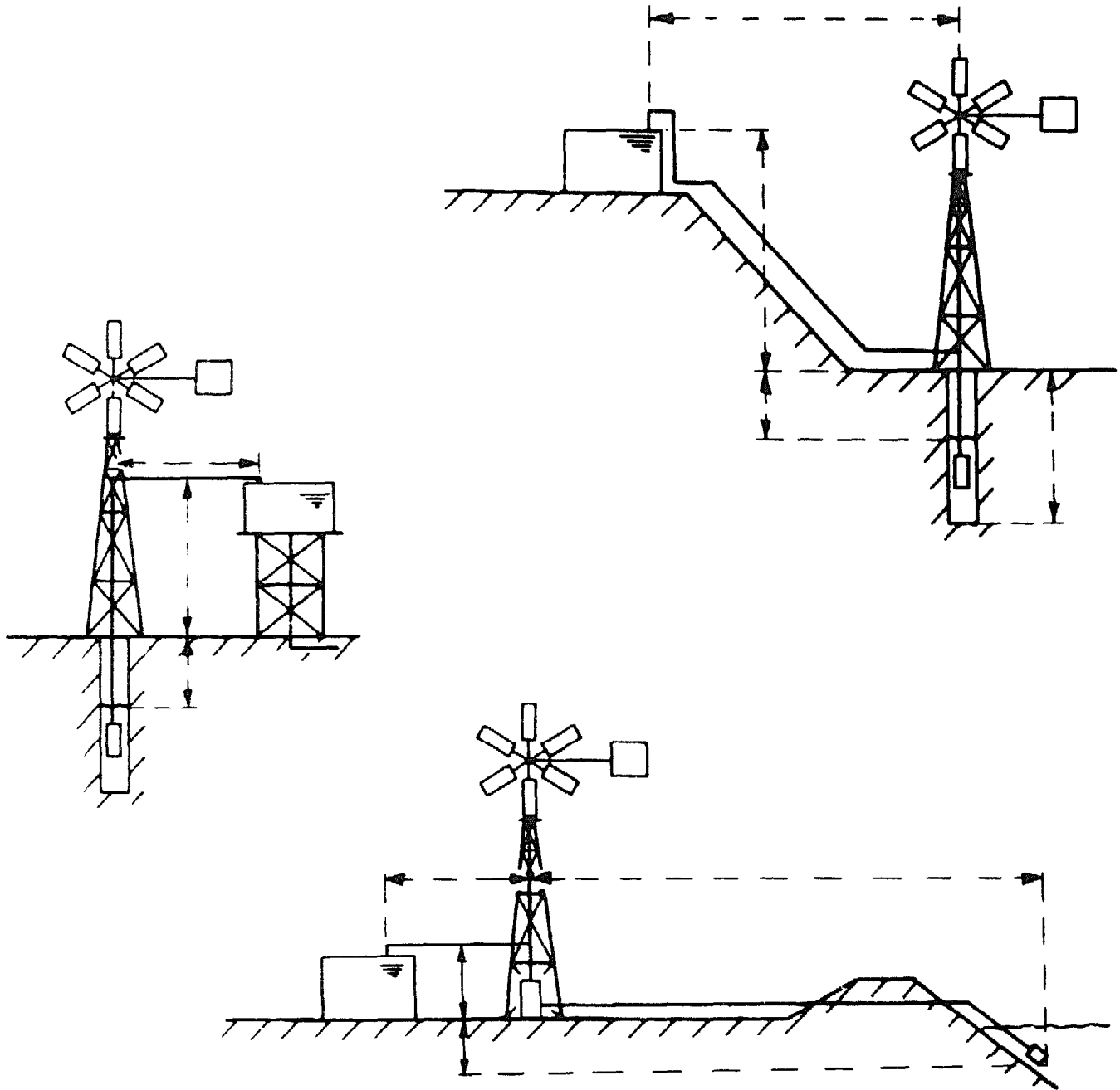
Figure F.1. Examples of layout of wind pumping systems. Indicate distances and heights for tender document.
