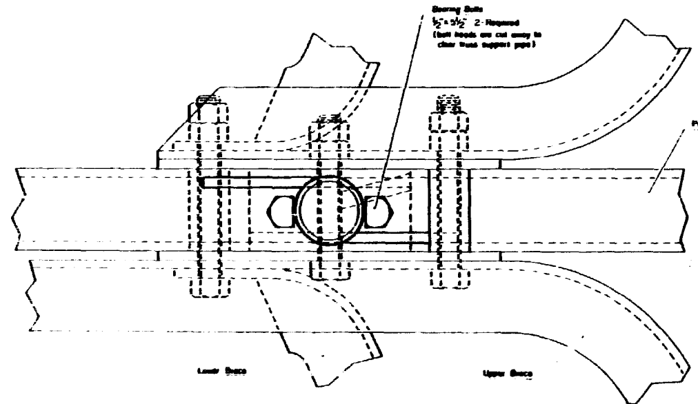
Top View - Lever Pivot Point
