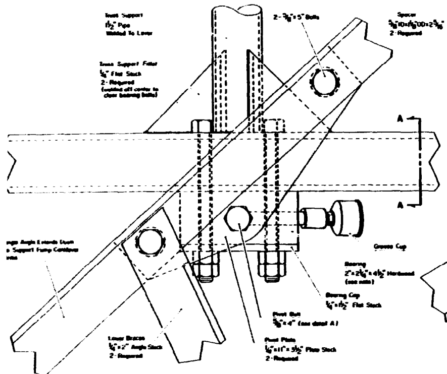
Side View - Lever Pivot Point
