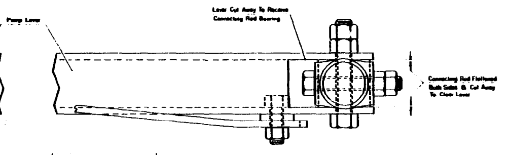
Top View - Lever End Pivot
