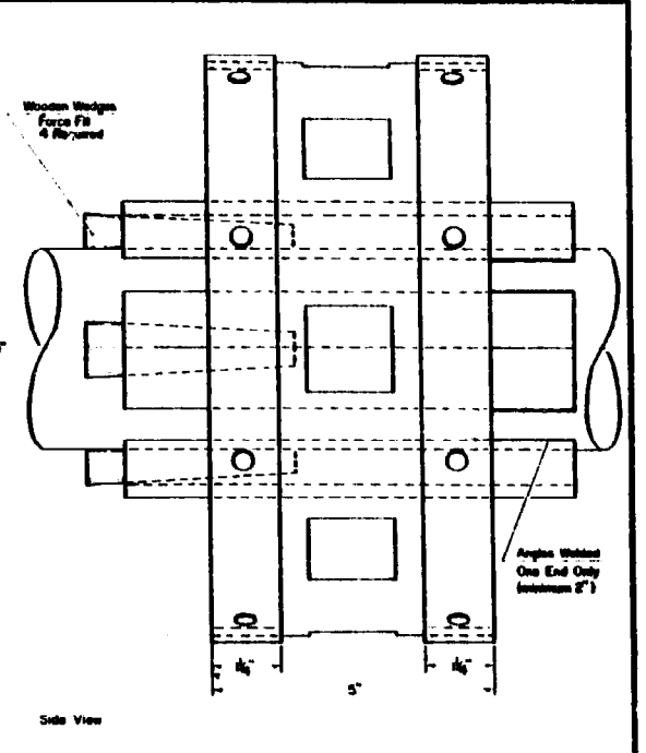
Hub Assembly Scale: Full Size
