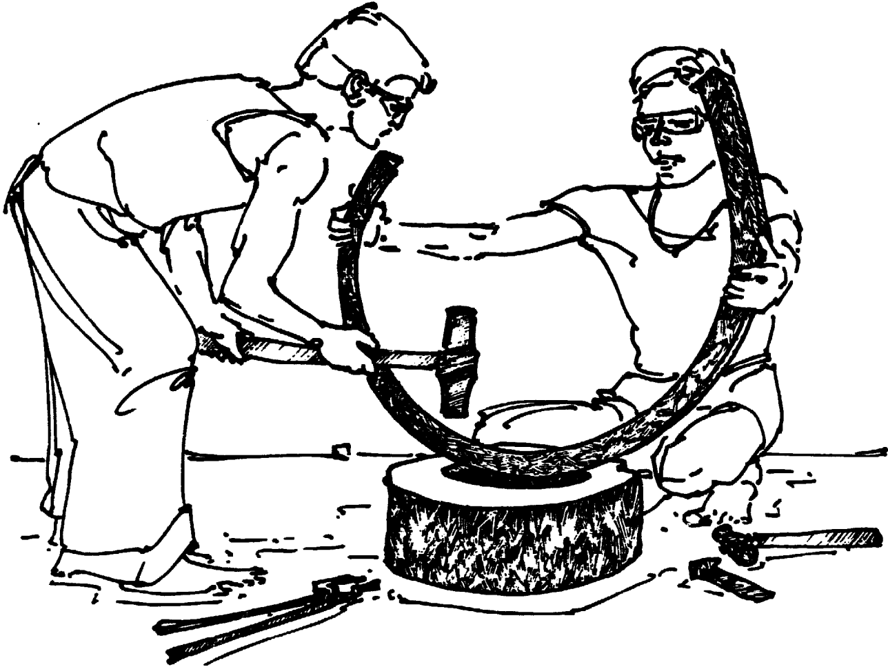
Figure 12. Bending the tower head ring
