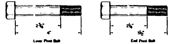
Detail A - Pivot Bolts
