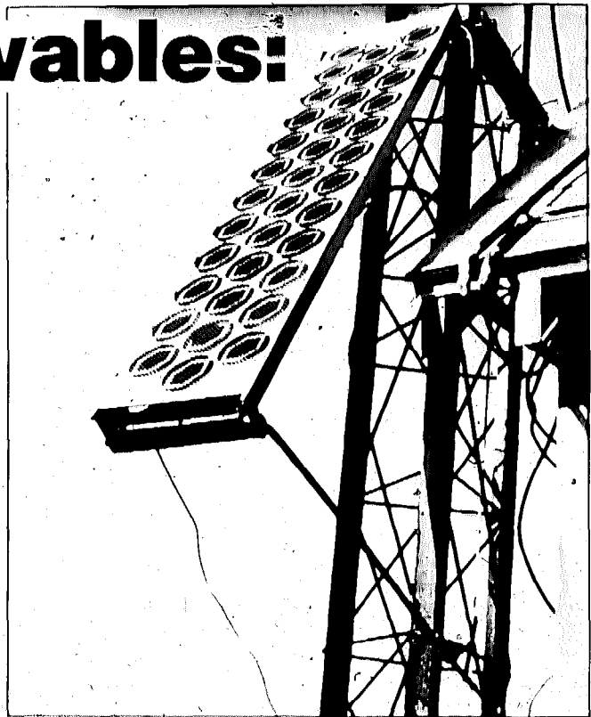
This photovoltaic panel's tilt angle can be changed in just seconds by loosening the wind-activated support bar. This system was designed by Richard B. Johnson of Columbia, Missouri, Arkansas. (A technical description of this system is given in this article and is on page 20 of the Wind & Sun , throughout Arkansas, including one courtesy from B&W with a PV system.)
