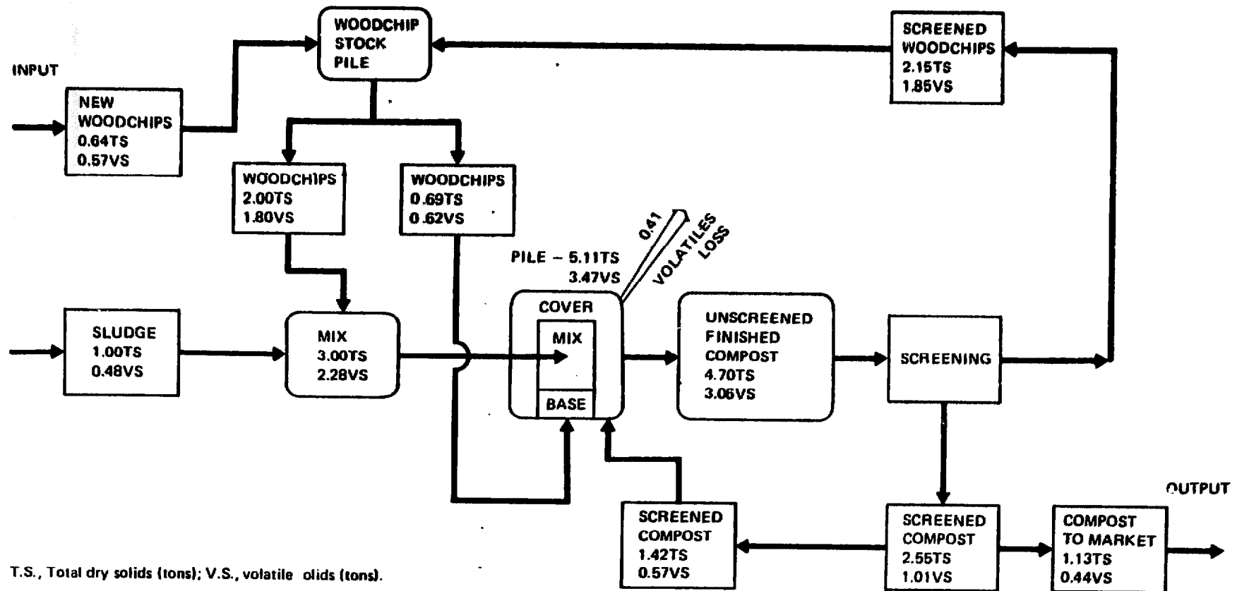
Figure 7. Materials Balance for the BARC System
