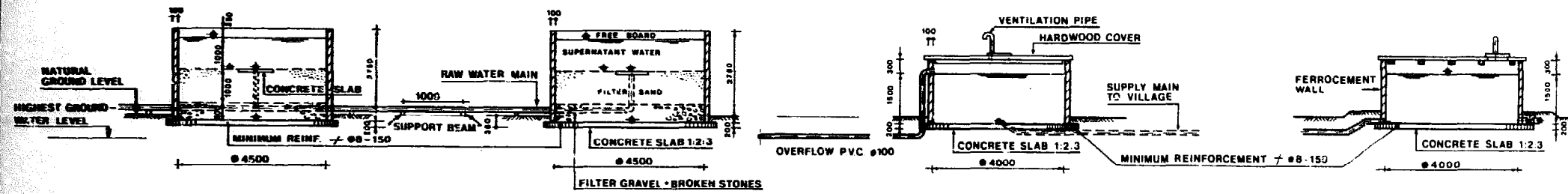
section C-C
