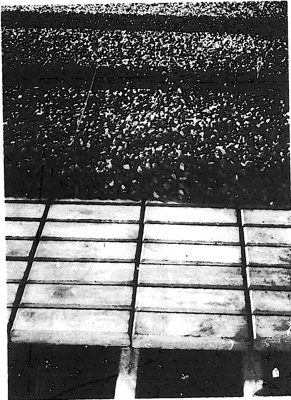
System of underdrains and supporting gravel layers, Amsterdam Waterworks, the Netherlands.
