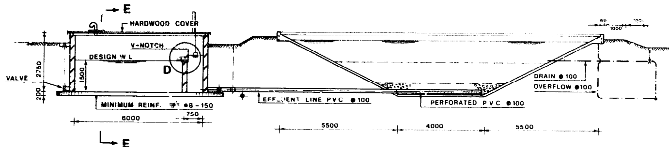
section B-B
