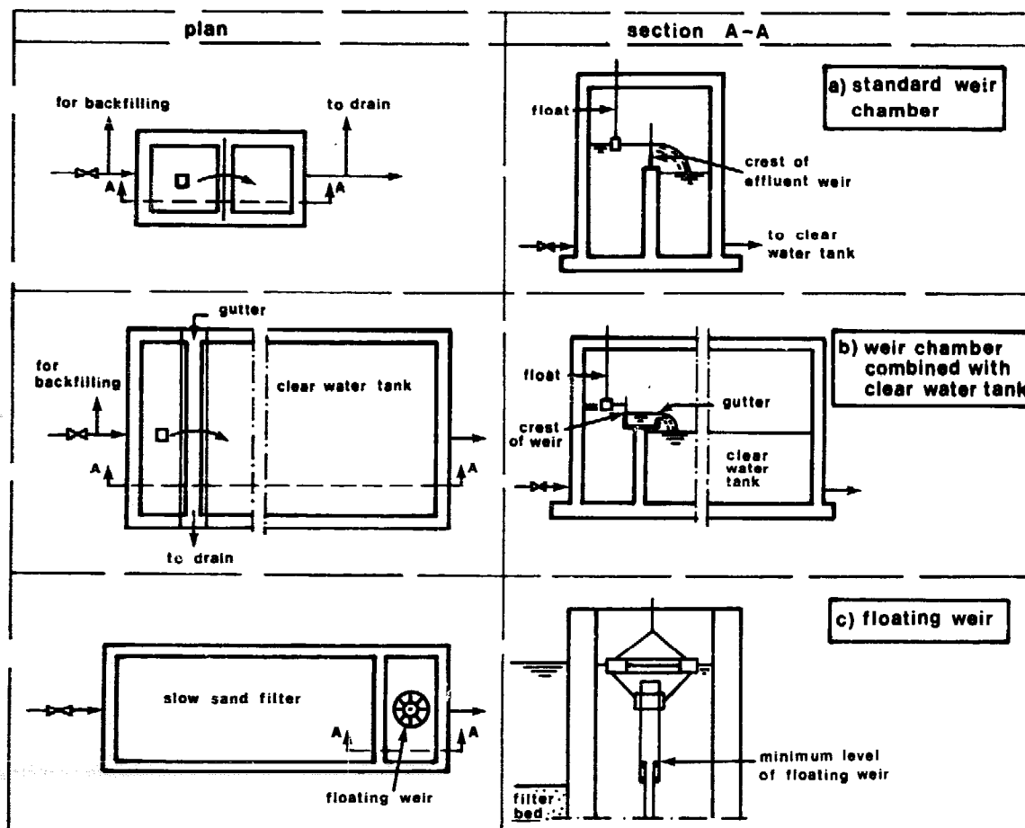
Figure 5.12. Outlet structures
