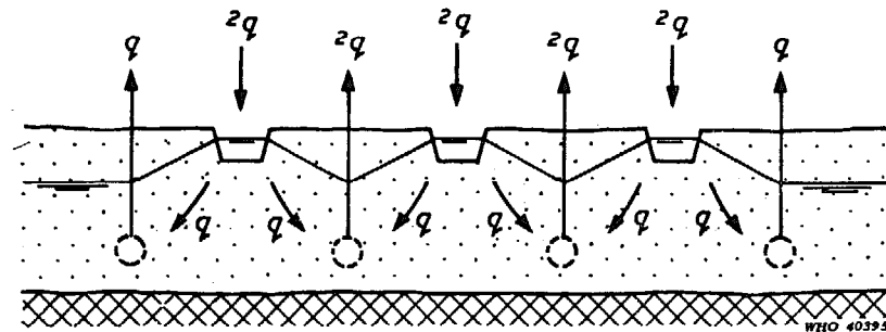
FIG. 43. ARTIFICIAL RECHARGE WITH DITCHES
