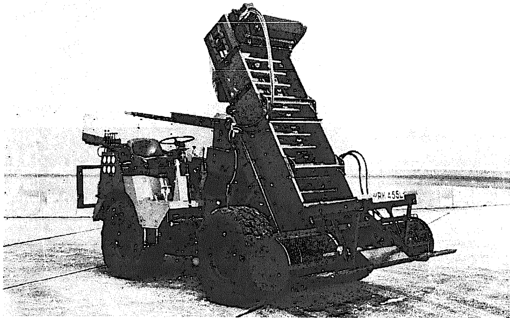
FIG. 33. TRACTOR-MOUNTED SKIMMER
