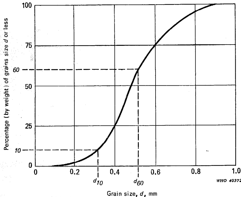
FIG. 5. SIEVE ANALYSIS
