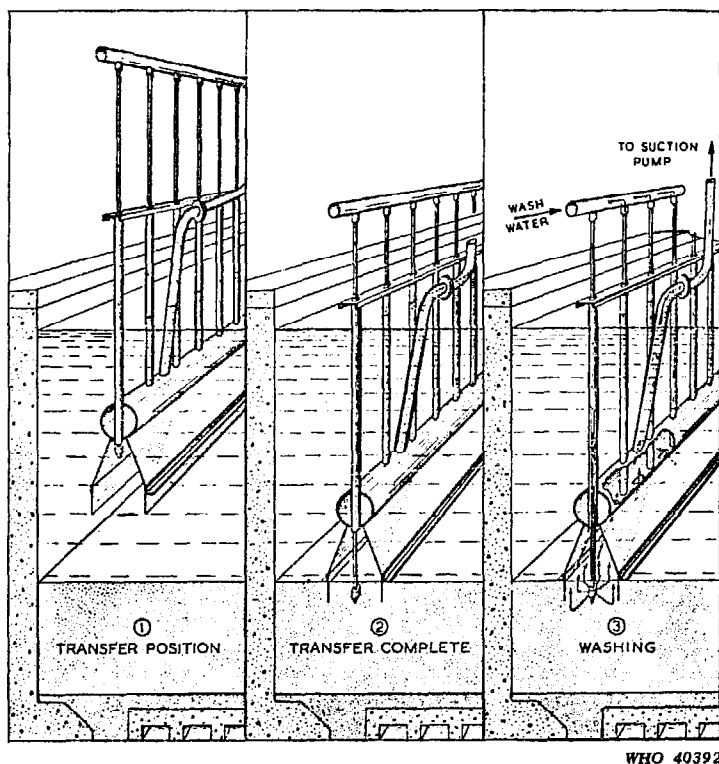
FIG. 40. SAND WASHING IN SITU : MODE OF OPERATION
