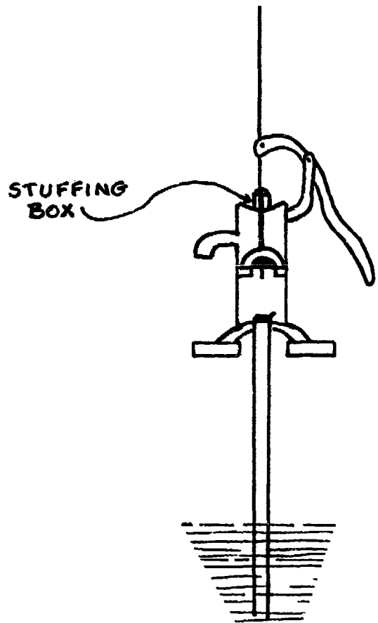
FIG. VII-4. SHALLOW WELL; LIFT AND FORCE PUMP
