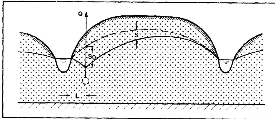
Figure 9.4. Induced recharge
