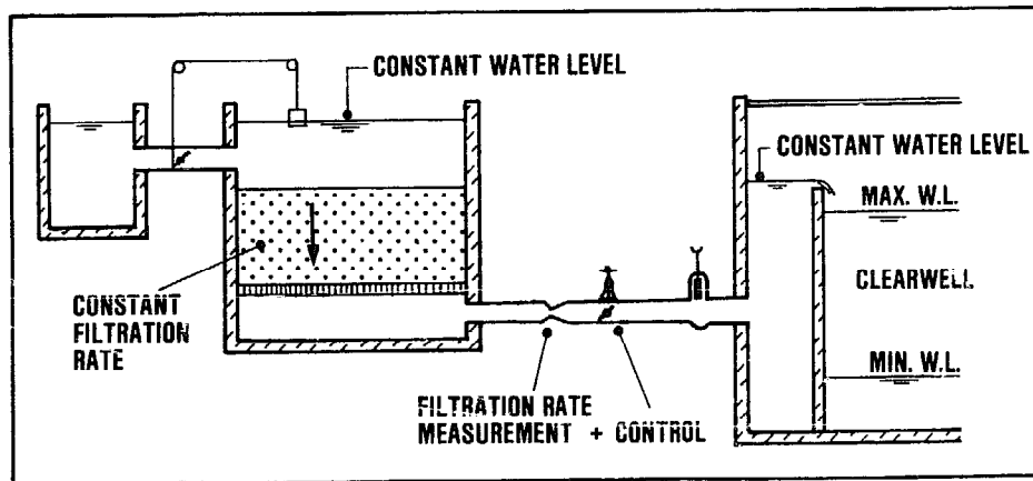
Figure 16.9. Filter-rate control
