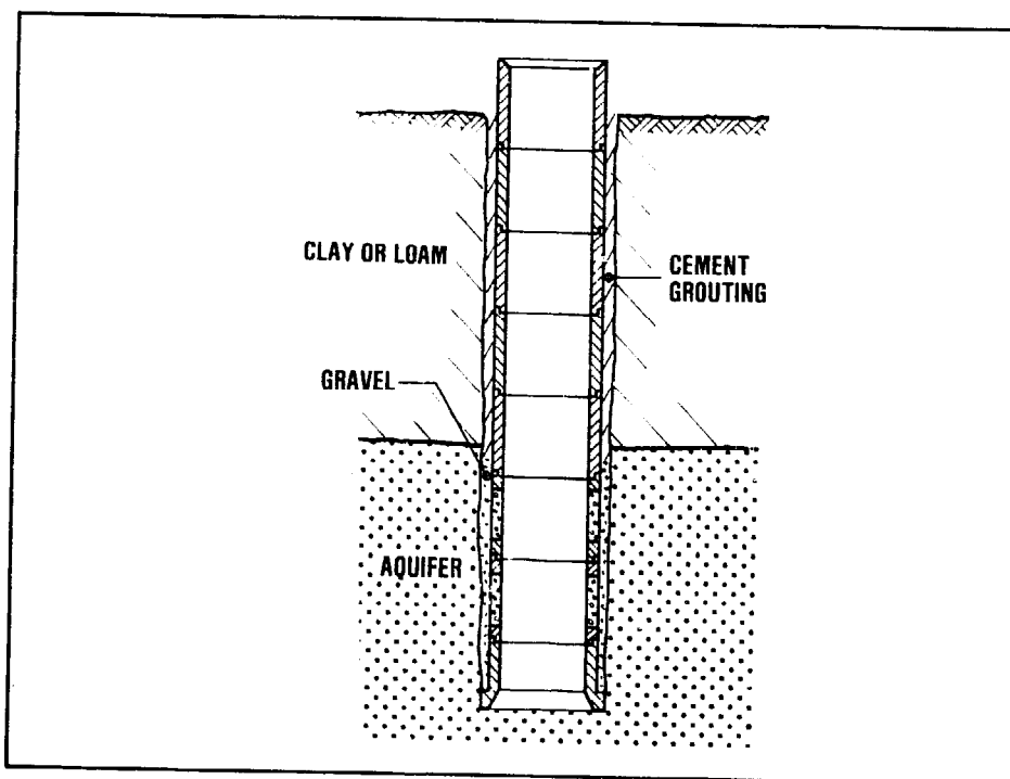
Figure 7.28. Dug well construction with pre-fabricated rings.
