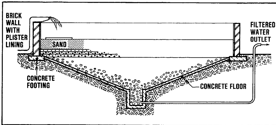
Figure 15.8. Simple slow sand filter
