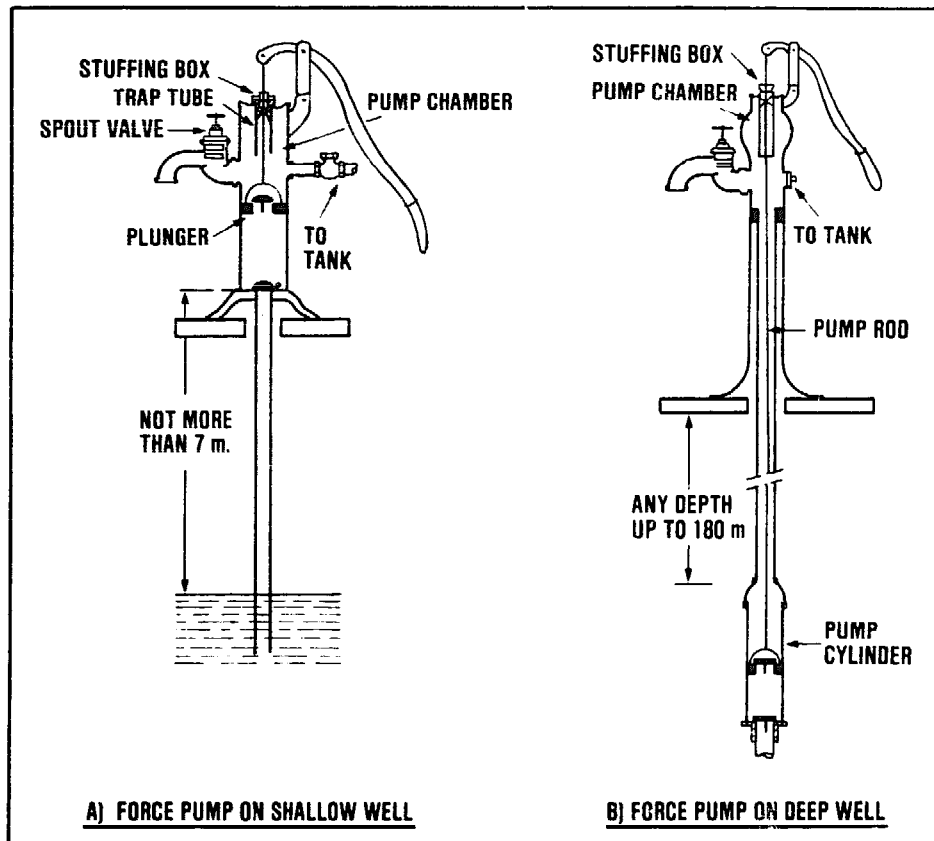
Figure 10.6. Force pumps
