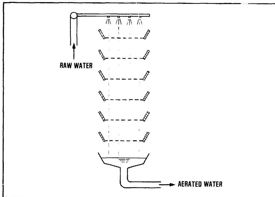
Figure 12.1. Multiple-tray aerator
