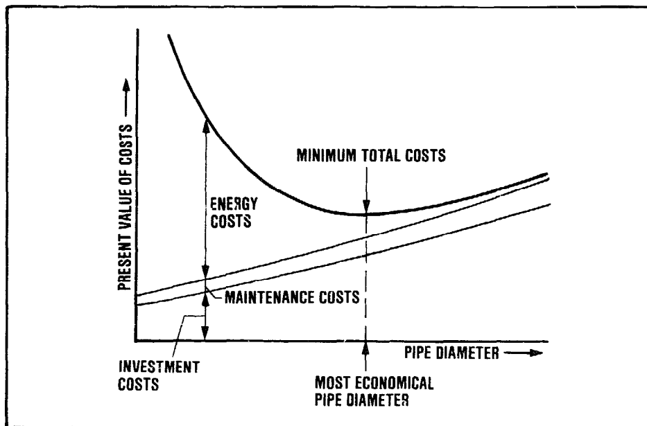
Figure 18.10. Determination of most economical pipe diameter
