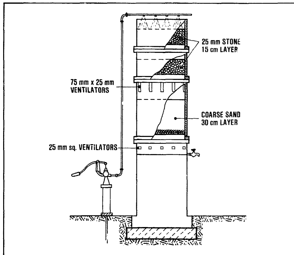
Figure 12.3. Hand-operated aeration/filtration unit
