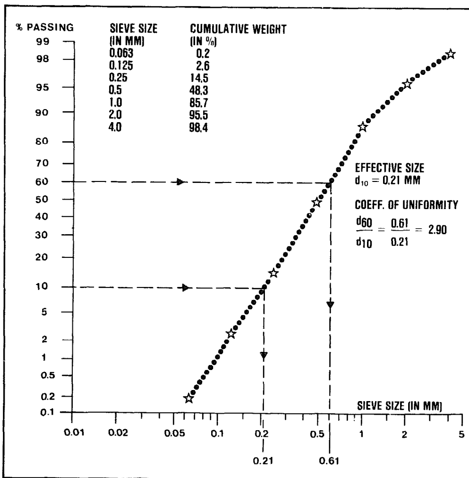
Figure 15.5. Grain size distribution of filter sand
