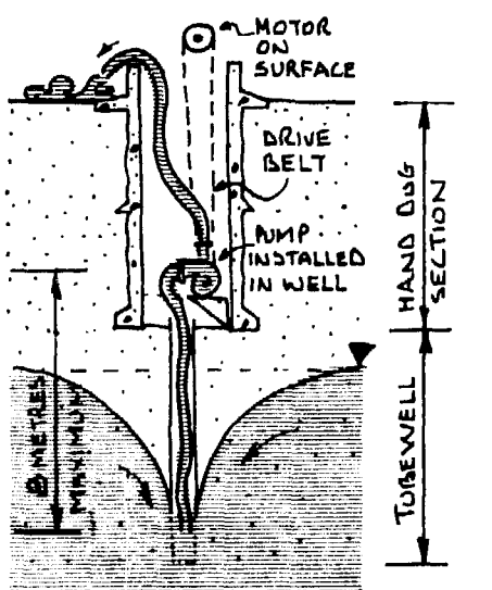
CENTRIFUGAL PUMP AT BASE OF HAND DUG SECTION EXTRACTING WATER FROM TUBEWELL
