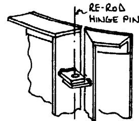
DETAIL OF EXTERIOR SHUTTER JOINING BRACKET
