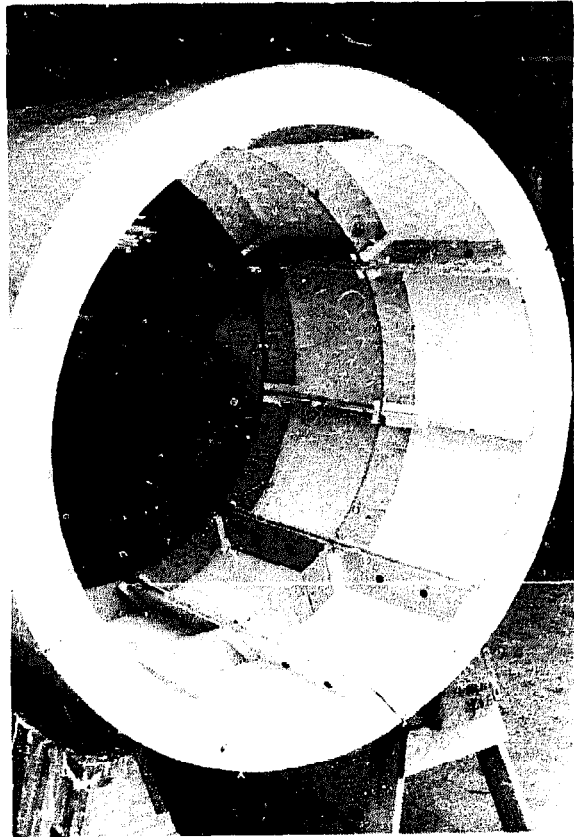
Photo 82 f) Adding lining sheet to assembled frame.
