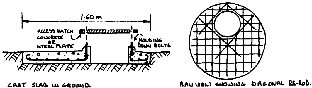
Construction of wellhead slab.
