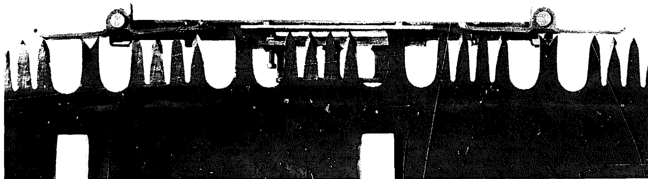
Jointing a saw with a long jointer.
