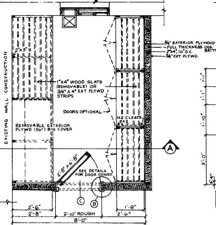
FLOOR PLAN SCALE: 1/2" = 1'-0"
