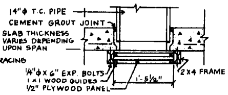
SLIDING DAMPER DETAIL SCALE: 3/4" = 1'-0"
