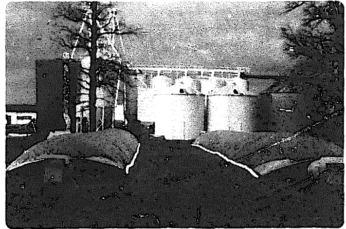
Figure 3.—Commercially available inflated plastic solar collectors used in tests at Purdue University.
