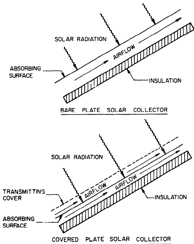
Figure 2.—Schematic of bare-plate and covered-plate solar collector for heating air.
