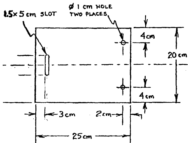
HASP PLATE (Make from barrel bottom)
