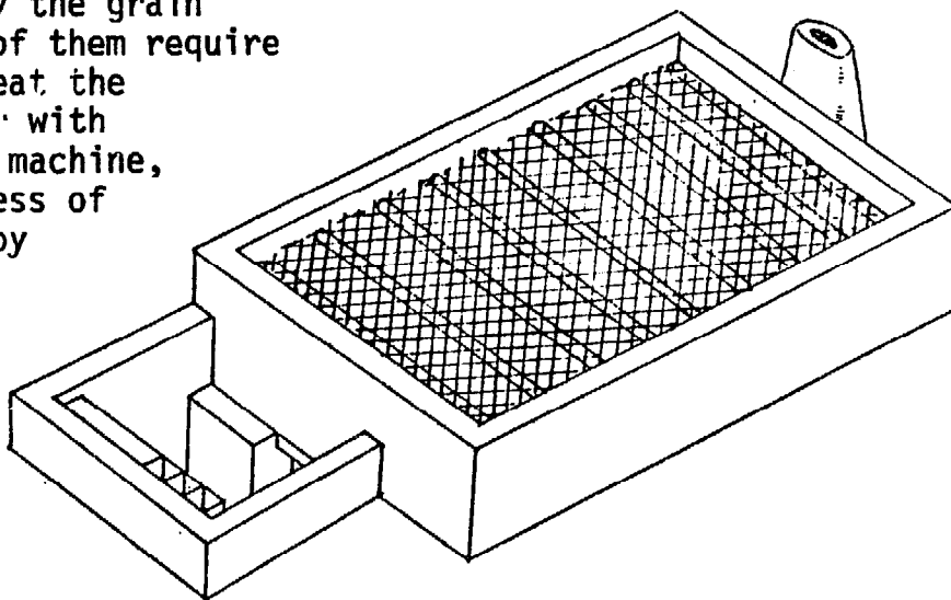
THE PIT OIL BARREL DRYER
