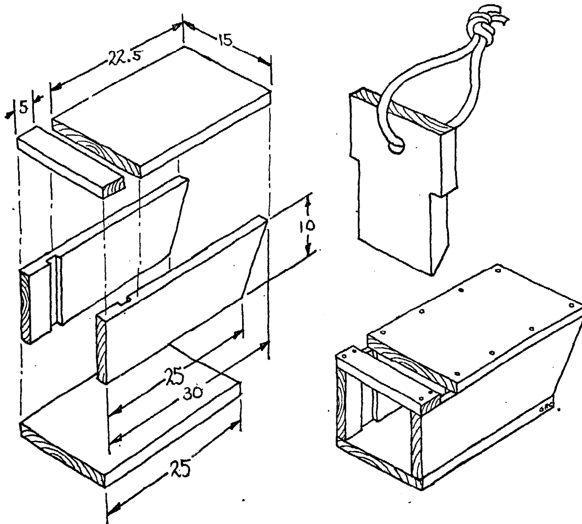
GRAIN CHUTE
