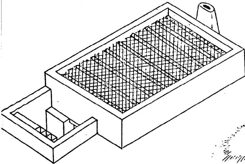
Pit Barrel Dryer
