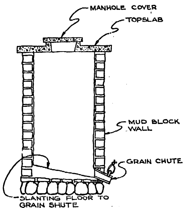
SECTION VIEW THROUGH MUD BLOCK SILO
