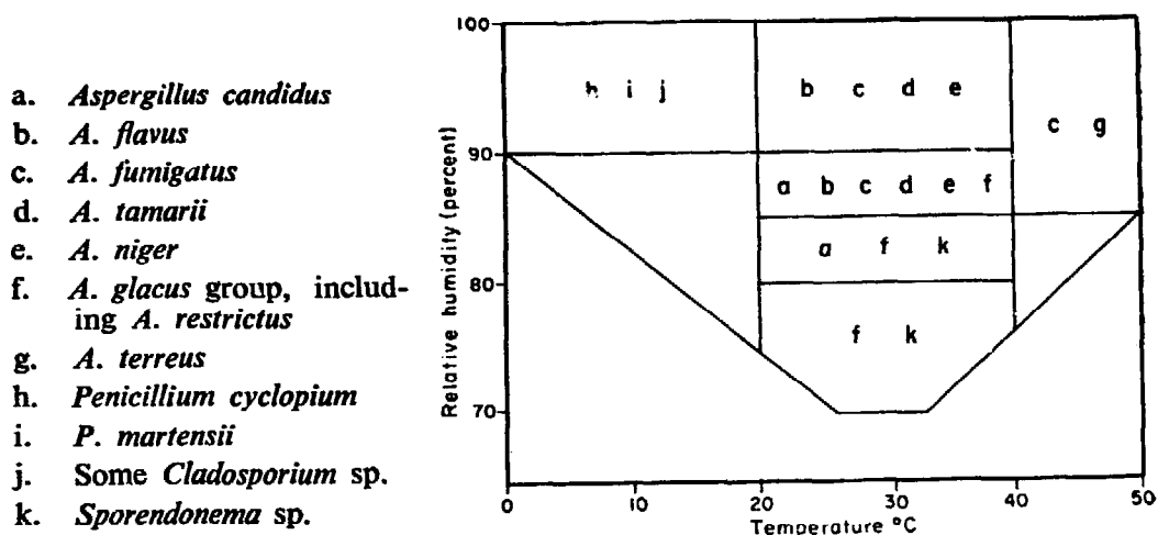
FIGURE 12. Effect of temperature and relative humidity on certain species of fungi.
