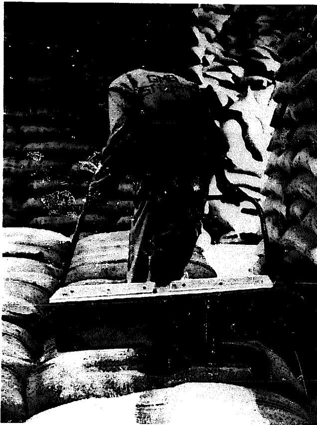
FIGURE 49. Insecticidal dust treatment. Top left, dusting each layer of bags as a stack is being built; top right, dusting the outside of a completed stack of bagged produce; left, a vertical drop duster for treating layers of bagged produce with insecticidal dust.
