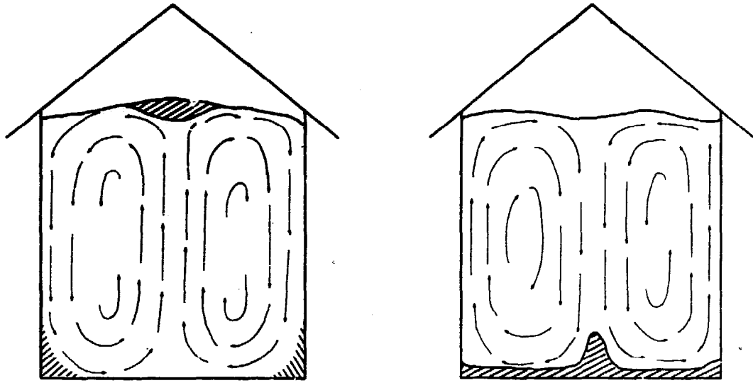
FIGURE 10. Moisture movement within bulk of grain due to differences between the temperature of outside air and of stored grain. Left, outside air temperature below grain temperature; right, outside air temperature above grain temperature.
