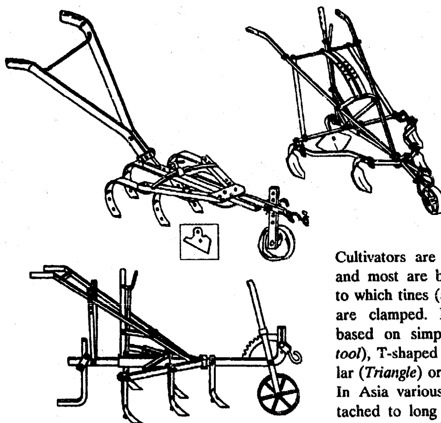
Fig. 7-38: Expandable cultivators. Top left: "Houe Manga" manufactured by UPRONA, Togo. Top right: "Rhino" cultivator manufactured by Northland Engineering, Zambia. Lower left: Interrow cultivator developed by CAMERTEC, Tanzania
