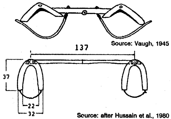
Fig. 4-10: Prototype collar-type yokes.
