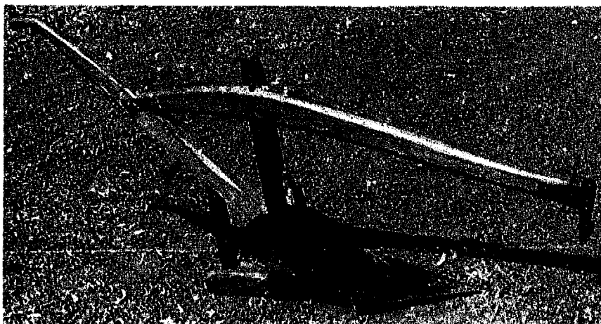
Fig. 7-10: Chinese single-handled, wooden "swing" plow with symmetrical cast-iron share.
