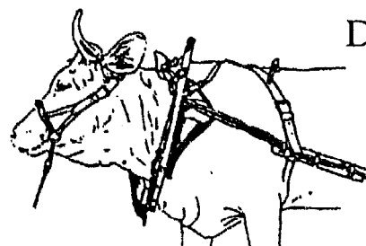
Fig. 4-3: Swiss independent harnessing systems for cattle. A - 3-point collar; B - Single withers yoke; C - Berne collar; D - 3-point collar.
