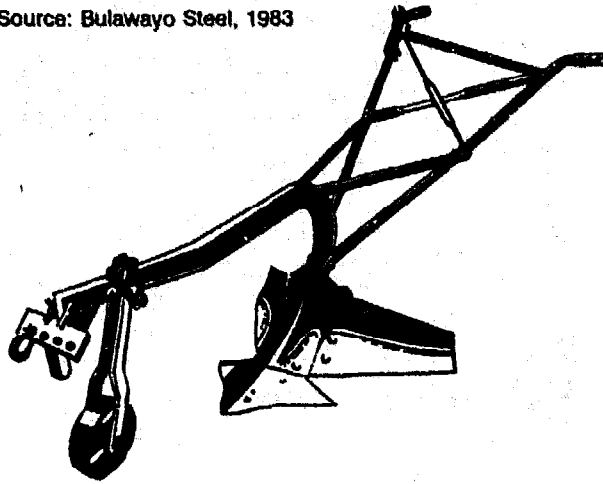
Fig. 7-21: "Inkanki" high wing ridger, manufactured in Zimbabwe.
