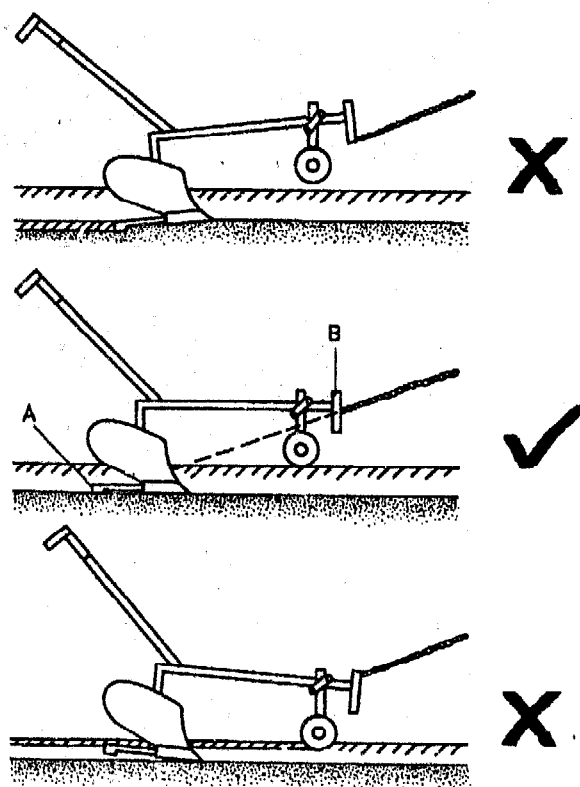
Fig. 2-5: Pitch adjustment of a plow (exaggerated).
