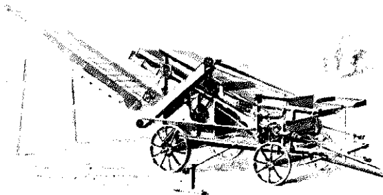
FIG. 10. RUSSELL & COMPANY'S "VINCENNE" DOUBLE PAN. PATENTED 1869.
