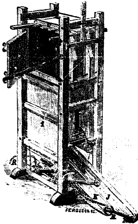
DEDERICK'S HAY-PRESS to $175, according to size. Made by W. M. DEERING & Co. of Albany.
