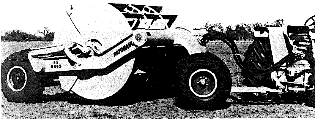
FIGURE 11. Rotary-type earth scraper which can be operated with a wheel tractor of 40-to-60-horsepower. The bowl has a capacity of 5 cubic metres.
