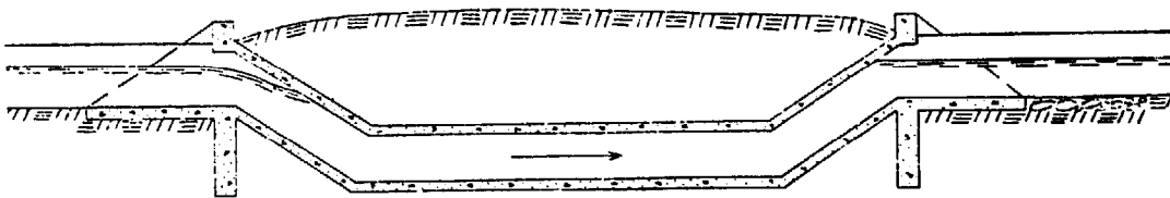
FIGURE 33. Cross-section of an inverted siphon placed under a roadway.
