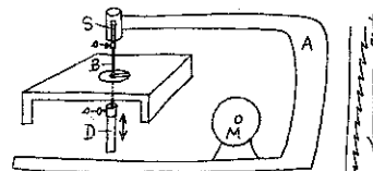
Schematic of JIG SAW M motor D drive a set screw B blade S spring A arm
