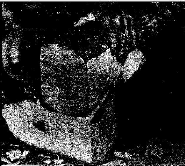
PLATE 72 Place the two together and check the fit. If not perfectly snug, shave off the high places using the axe as a chisel. To make the top log fit farther down on the bottom one, cut the notch deeper while maintaining the same slope.
