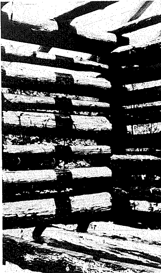
PLATE 97 The joists in Roy Thompson's cabin were lap-jointed to fit the plates. Note that the sleepers (bottom) and joists (top) are parallel.
