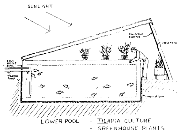
Fig. 13 Greenhouse - Fish Culture Structure
